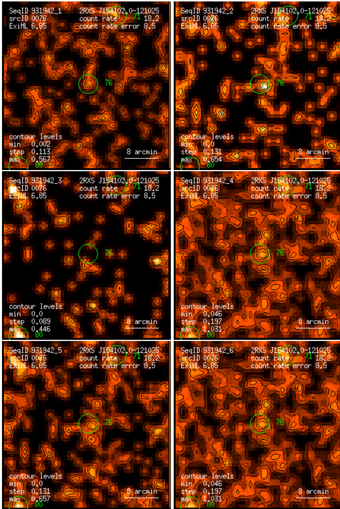
Figure 76: RASS 931942: detection 0076: band rate images, Gaussian filter: (1) PSPC channels 11 – 41, (2) 52 – 90, (3) 91 – 201, (4) 11 – 235, (5) 52 – 201, (6) 11 – 201. Broad band rates in counts/ks. Band rate contour levels in counts/ks/arcmin 2 .
