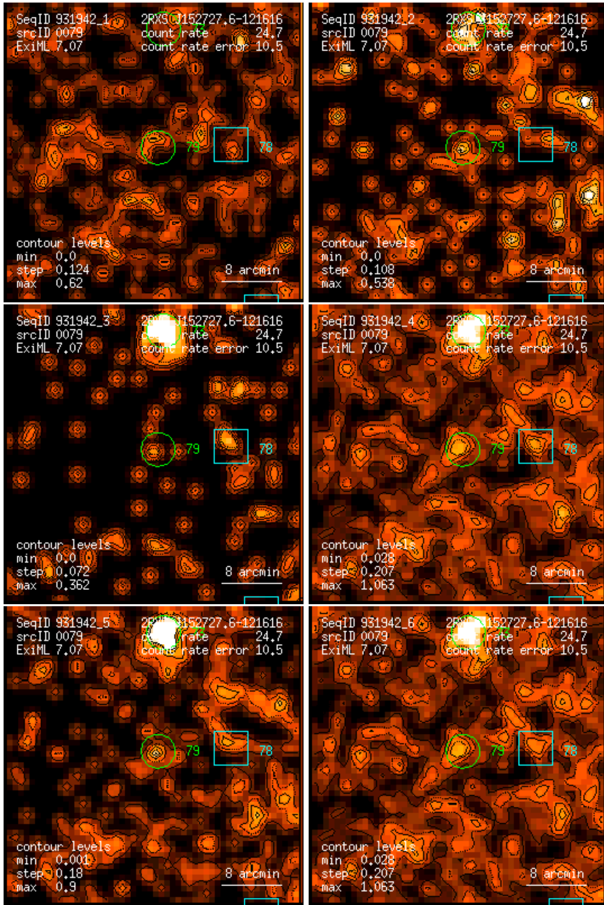
Figure 79: RASS 931942: detection 0079: band rate images, Gaussian filter: (1) PSPC channels 11 – 41, (2) 52 – 90, (3) 91 – 201, (4) 11 – 235, (5) 52 – 201, (6) 11 – 201. Broad band rates in counts/ks. Band rate contour levels in counts/ks/arcmin 2 .
