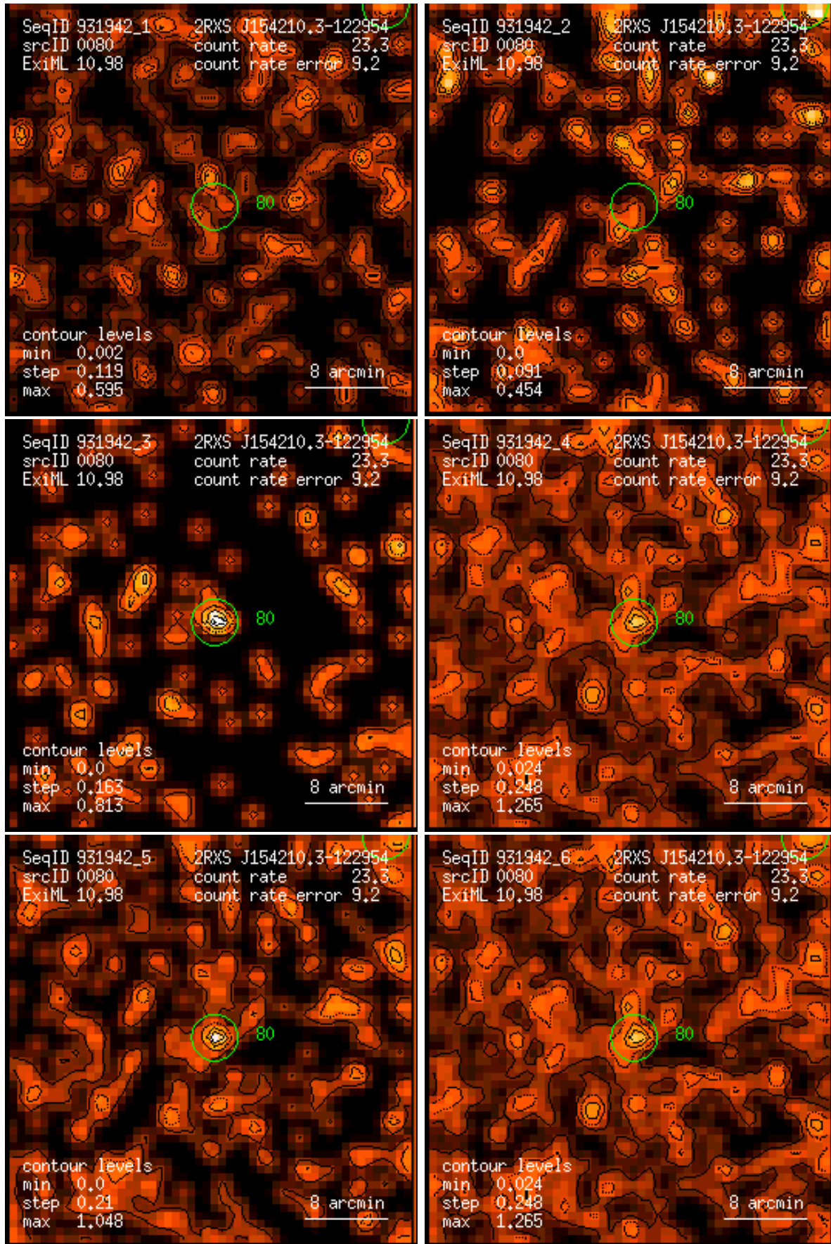
Figure 80: RASS 931942: detection 0080: band rate images, Gaussian filter: (1) PSPC channels 11 – 41, (2) 52 – 90, (3) 91 – 201, (4) 11 – 235, (5) 52 – 201, (6) 11 – 201. Broad band rates in counts/ks. Band rate contour levels in counts/ks/arcmin 2 .
