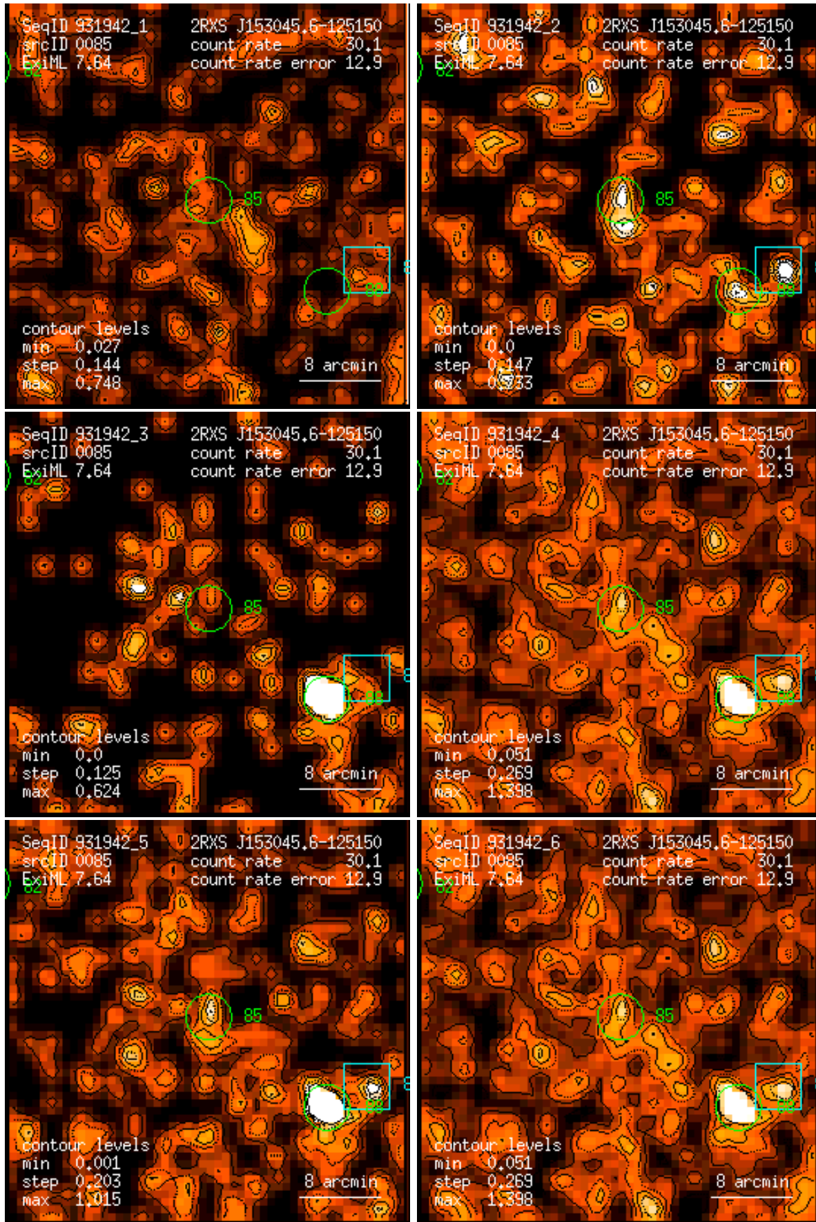
Figure 85: RASS 931942: detection 0085: band rate images, Gaussian filter: (1) PSPC channels 11 – 41, (2) 52 – 90, (3) 91 – 201, (4) 11 – 235, (5) 52 – 201, (6) 11 – 201. Broad band rates in counts/ks. Band rate contour levels in counts/ks/arcmin 2 .
