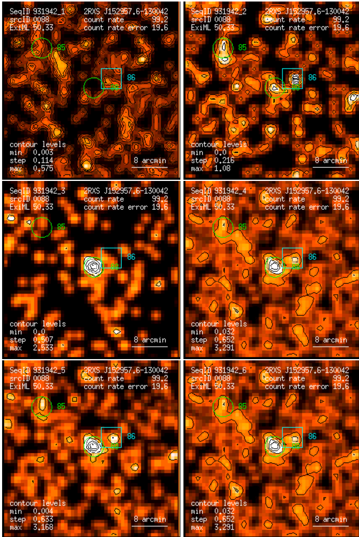
Figure 88: RASS 931942: detection 0088: band rate images, Gaussian filter: (1) PSPC channels 11 – 41, (2) 52 – 90, (3) 91 – 201, (4) 11 – 235, (5) 52 – 201, (6) 11 – 201. Broad band rates in counts/ks. Band rate contour levels in counts/ks/arcmin 2 .
