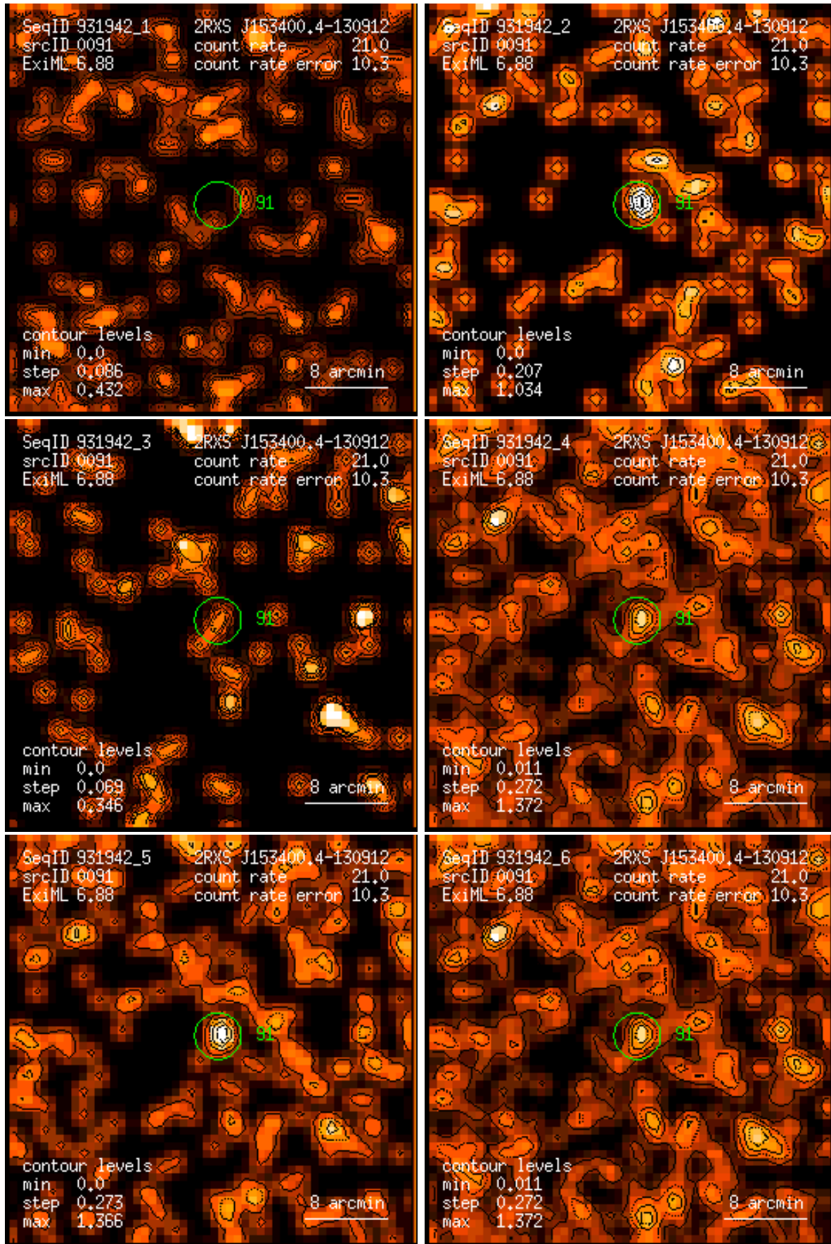
Figure 91: RASS 931942: detection 0091: band rate images, Gaussian filter: (1) PSPC channels 11 – 41, (2) 52 – 90, (3) 91 – 201, (4) 11 – 235, (5) 52 – 201, (6) 11 – 201. Broad band rates in counts/ks. Band rate contour levels in counts/ks/arcmin 2 .
