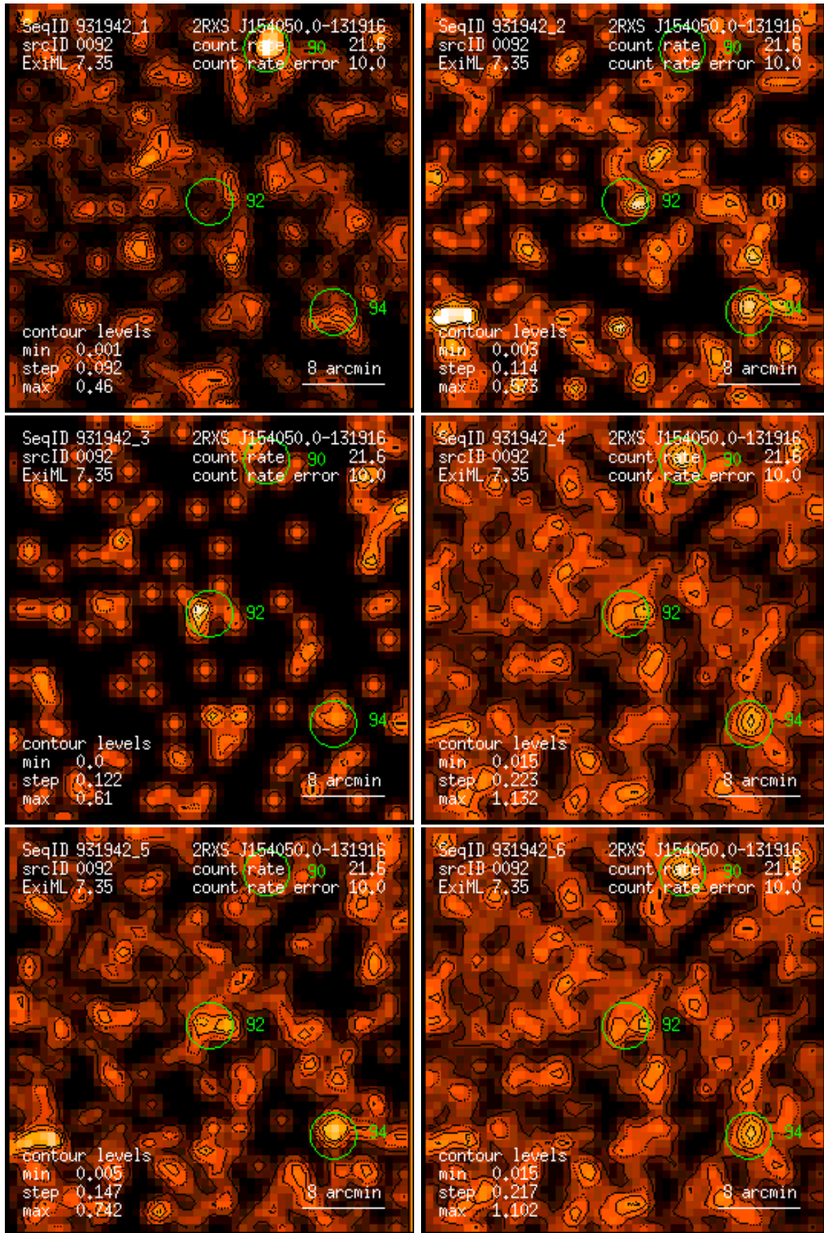
Figure 92: RASS 931942: detection 0092: band rate images, Gaussian filter: (1) PSPC channels 11 – 41, (2) 52 – 90, (3) 91 – 201, (4) 11 – 235, (5) 52 – 201, (6) 11 – 201. Broad band rates in counts/ks. Band rate contour levels in counts/ks/arcmin 2 .
