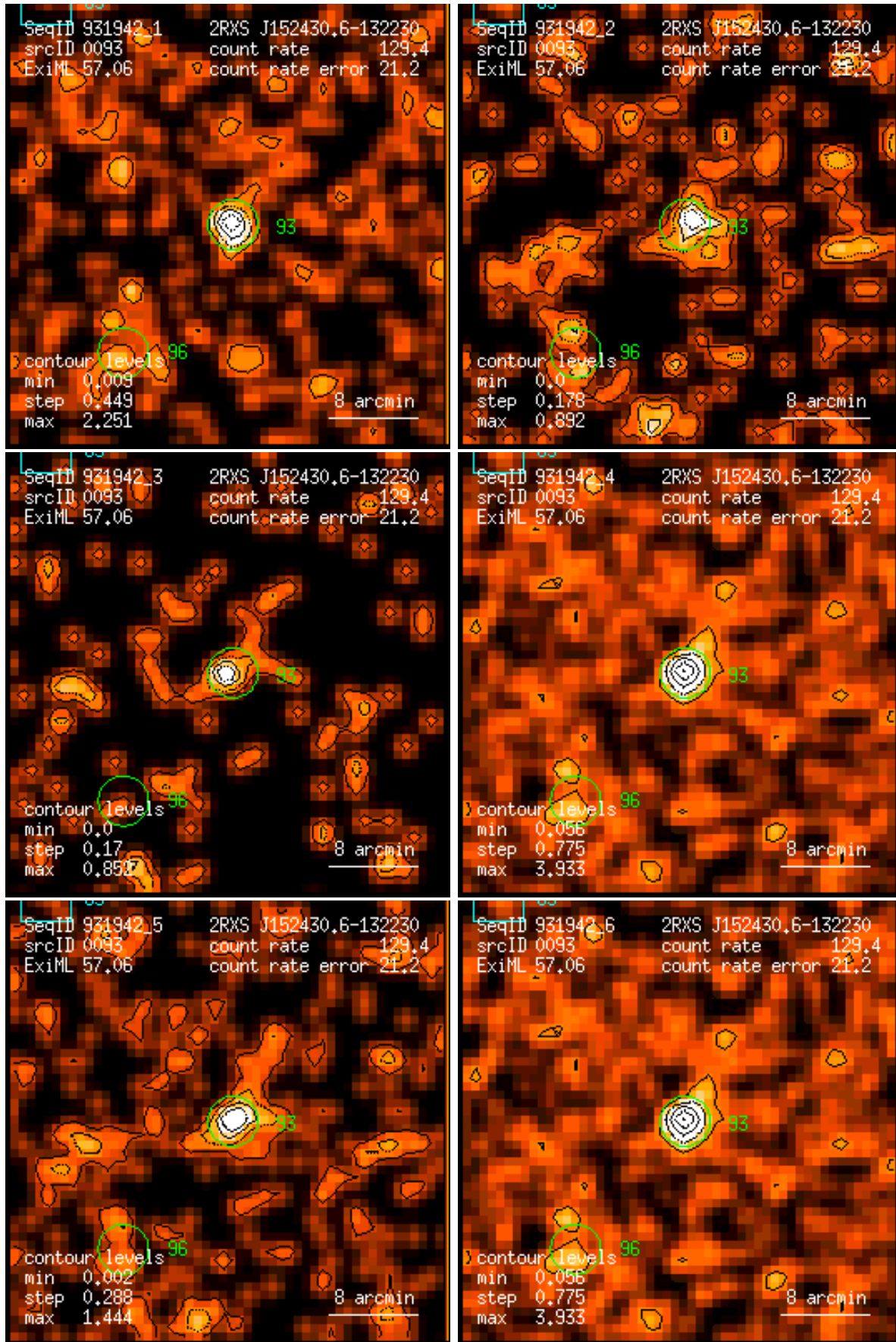
Figure 93: RASS 931942: detection 0093: band rate images, Gaussian filter: (1) PSPC channels 11 – 41, (2) 52 – 90, (3) 91 – 201, (4) 11 – 235, (5) 52 – 201, (6) 11 – 201. Broad band rates in counts/ks. Band rate contour levels in counts/ks/arcmin 2 .
