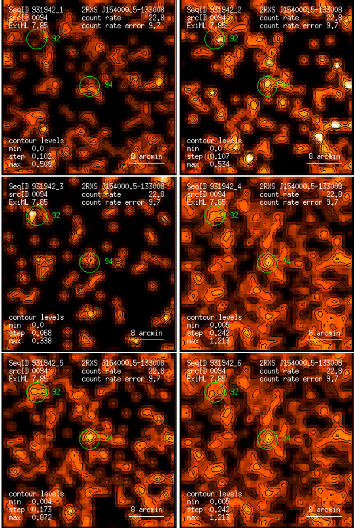
Figure 94: RASS 931942: detection 0094: band rate images, Gaussian filter: (1) PSPC channels 11 – 41, (2) 52 – 90, (3) 91 – 201, (4) 11 – 235, (5) 52 – 201, (6) 11 – 201. Broad band rates in counts/ks. Band rate contour levels in counts/ks/arcmin 2 .
