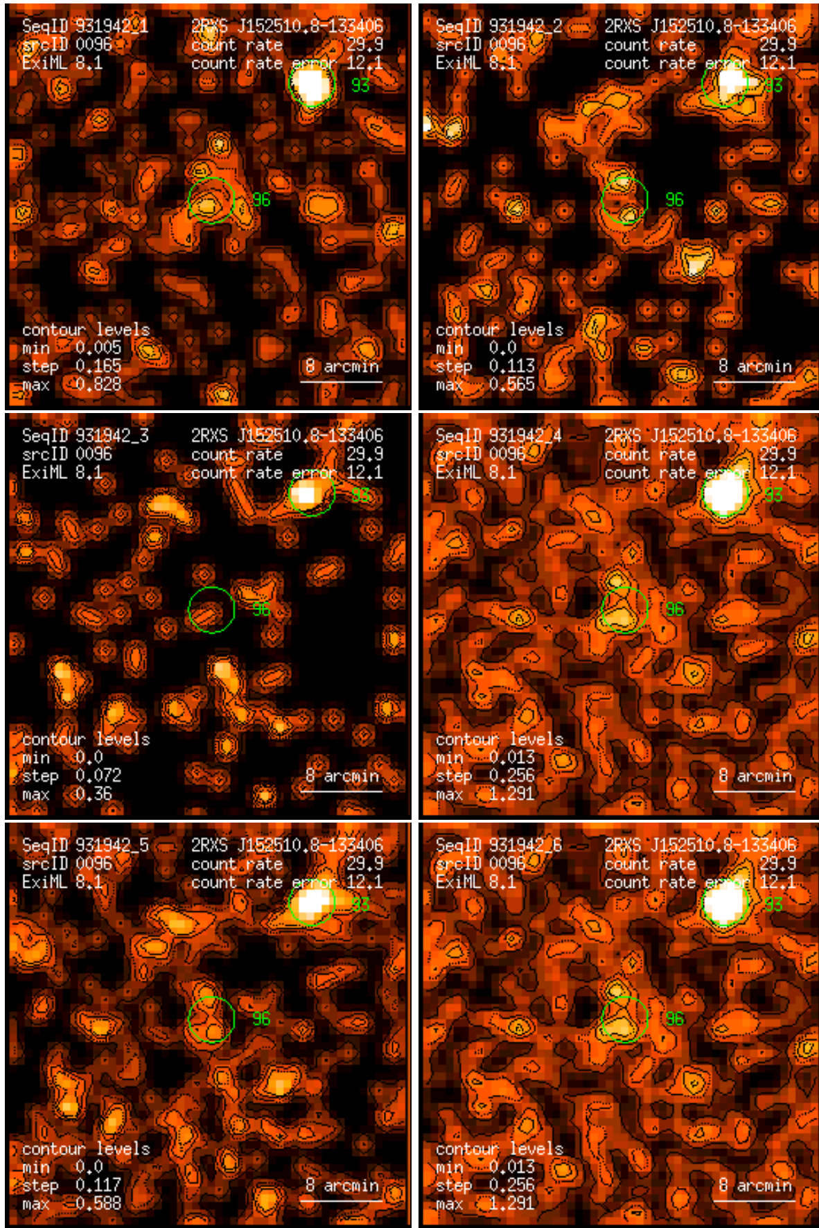
Figure 96: RASS 931942: detection 0096: band rate images, Gaussian filter: (1) PSPC channels 11 – 41, (2) 52 – 90, (3) 91 – 201, (4) 11 – 235, (5) 52 – 201, (6) 11 – 201. Broad band rates in counts/ks. Band rate contour levels in counts/ks/arcmin 2 .
