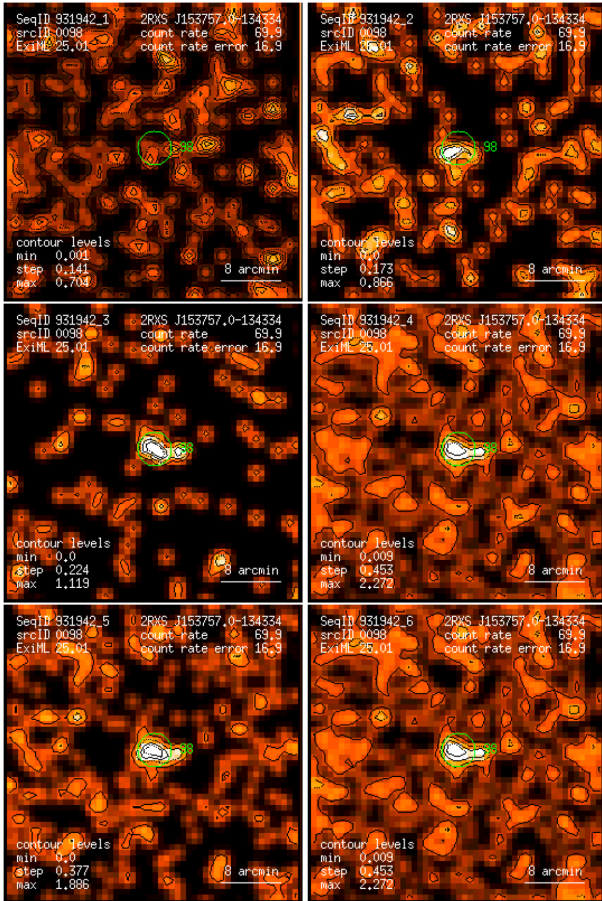
Figure 98: RASS 931942: detection 0098: band rate images, Gaussian filter: (1) PSPC channels 11 – 41, (2) 52 – 90, (3) 91 – 201, (4) 11 – 235, (5) 52 – 201, (6) 11 – 201. Broad band rates in counts/ks. Band rate contour levels in counts/ks/arcmin 2 .
