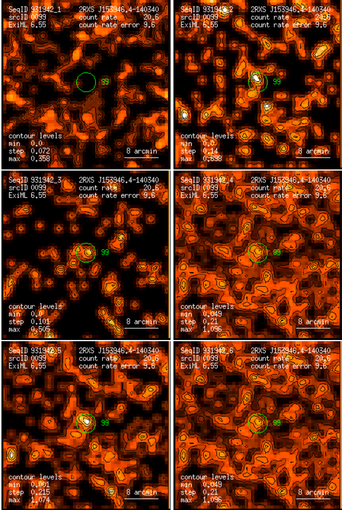
Figure 99: RASS 931942: detection 0099: band rate images, Gaussian filter: (1) PSPC channels 11 – 41, (2) 52 – 90, (3) 91 – 201, (4) 11 – 235, (5) 52 – 201, (6) 11 – 201. Broad band rates in counts/ks. Band rate contour levels in counts/ks/arcmin 2 .
