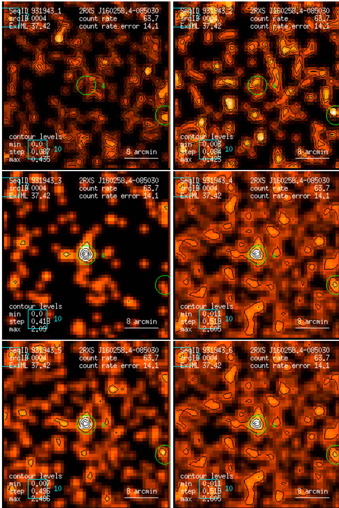
Figure 4: RASS 931943: detection 0004: band rate images, Gaussian filter: (1) PSPC channels 11 – 41, (2) 52 – 90, (3) 91 – 201, (4) 11 – 235, (5) 52 – 201, (6) 11 – 201. Broad band rates in counts/ks. Band rate contour levels in counts/ks/arcmin 2 .
