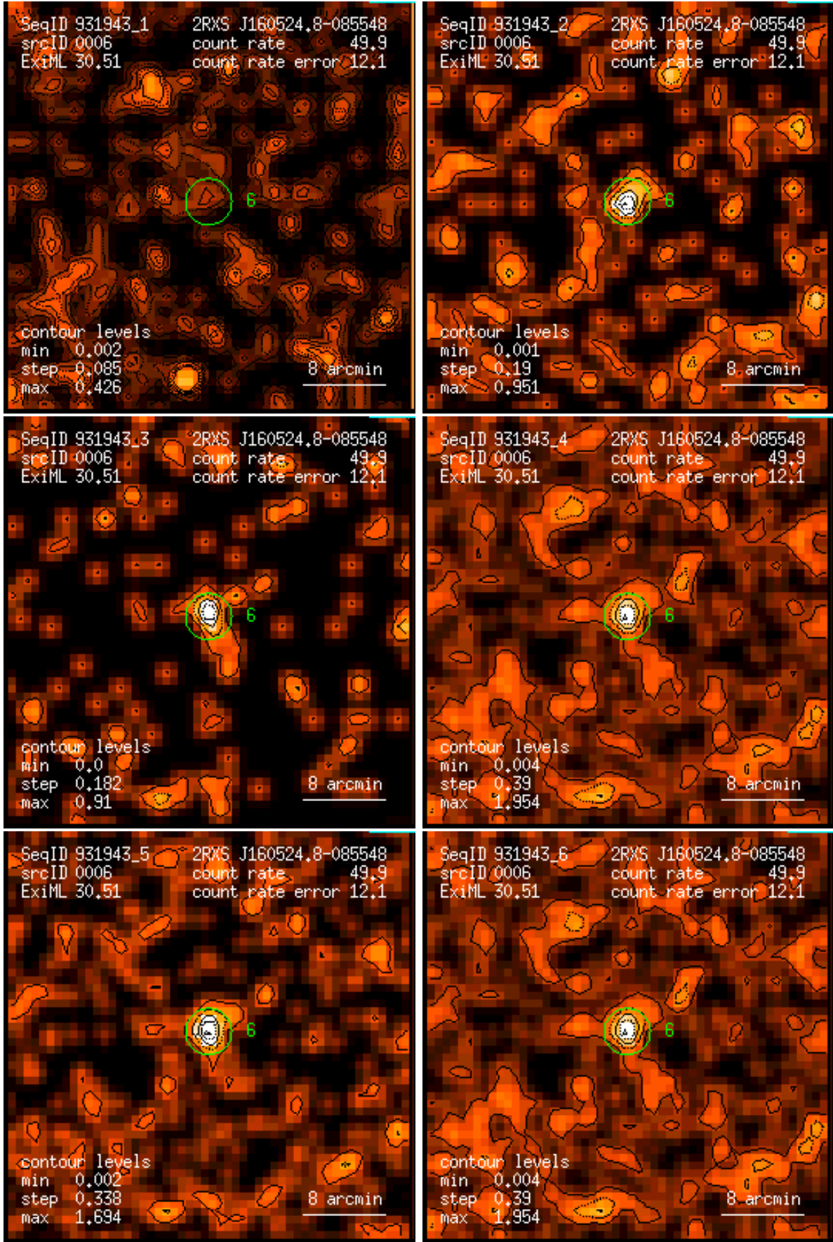
Figure 6: RASS 931943: detection 0006: band rate images, Gaussian filter: (1) PSPC channels 11 – 41, (2) 52 – 90, (3) 91 – 201, (4) 11 – 235, (5) 52 – 201, (6) 11 – 201. Broad band rates in counts/ks. Band rate contour levels in counts/ks/arcmin 2 .
