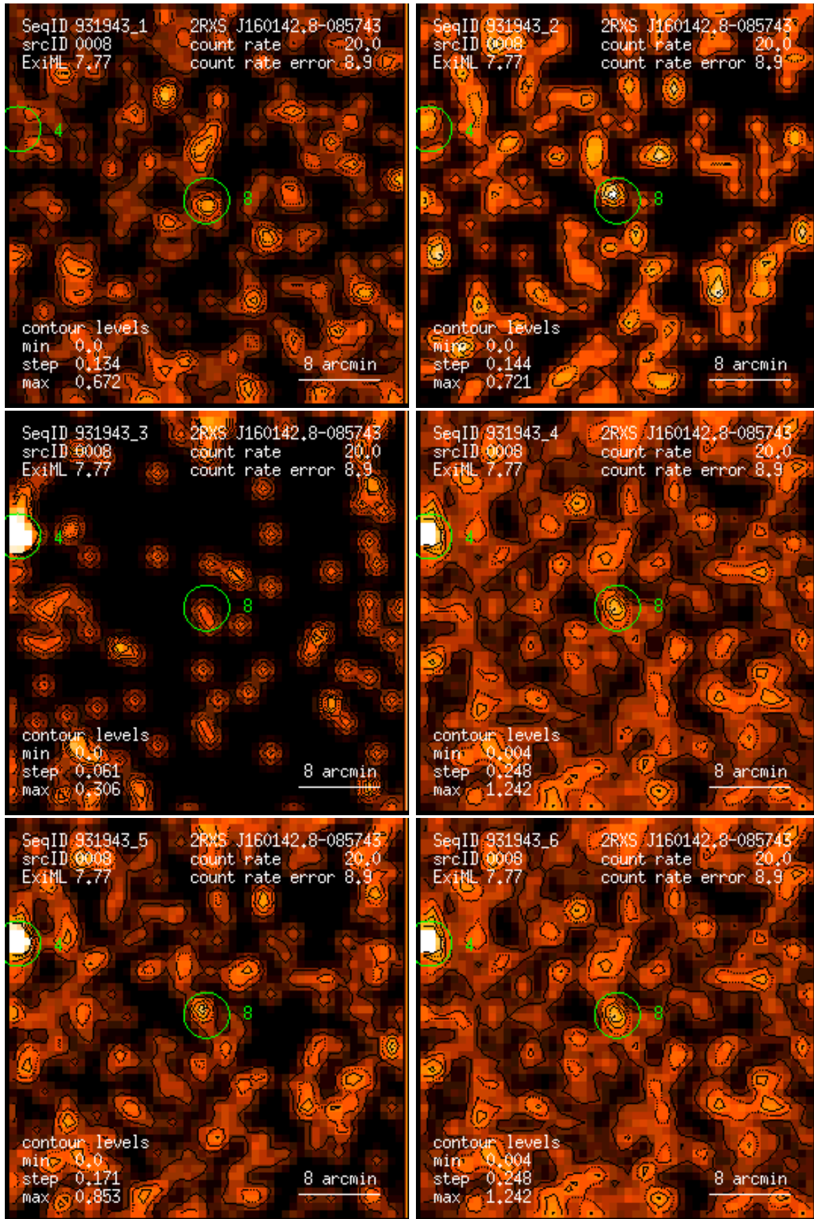
Figure 8: RASS 931943: detection 0008: band rate images, Gaussian filter: (1) PSPC channels 11 – 41, (2) 52 – 90, (3) 91 – 201, (4) 11 – 235, (5) 52 – 201, (6) 11 – 201. Broad band rates in counts/ks. Band rate contour levels in counts/ks/arcmin 2 .
