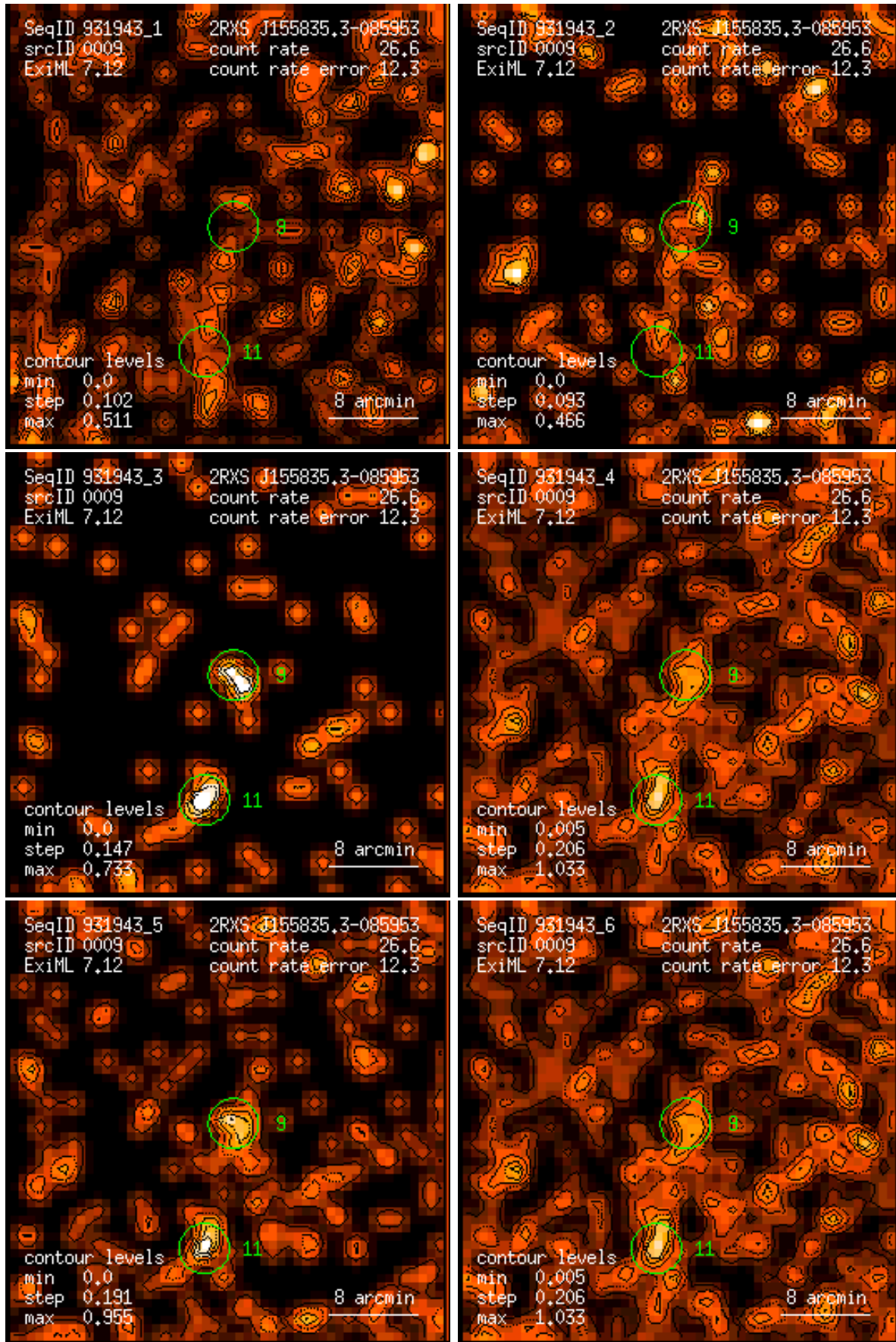
Figure 9: RASS 931943: detection 0009: band rate images, Gaussian filter: (1) PSPC channels 11 – 41, (2) 52 – 90, (3) 91 – 201, (4) 11 – 235, (5) 52 – 201, (6) 11 – 201. Broad band rates in counts/ks. Band rate contour levels in counts/ks/arcmin 2 .
