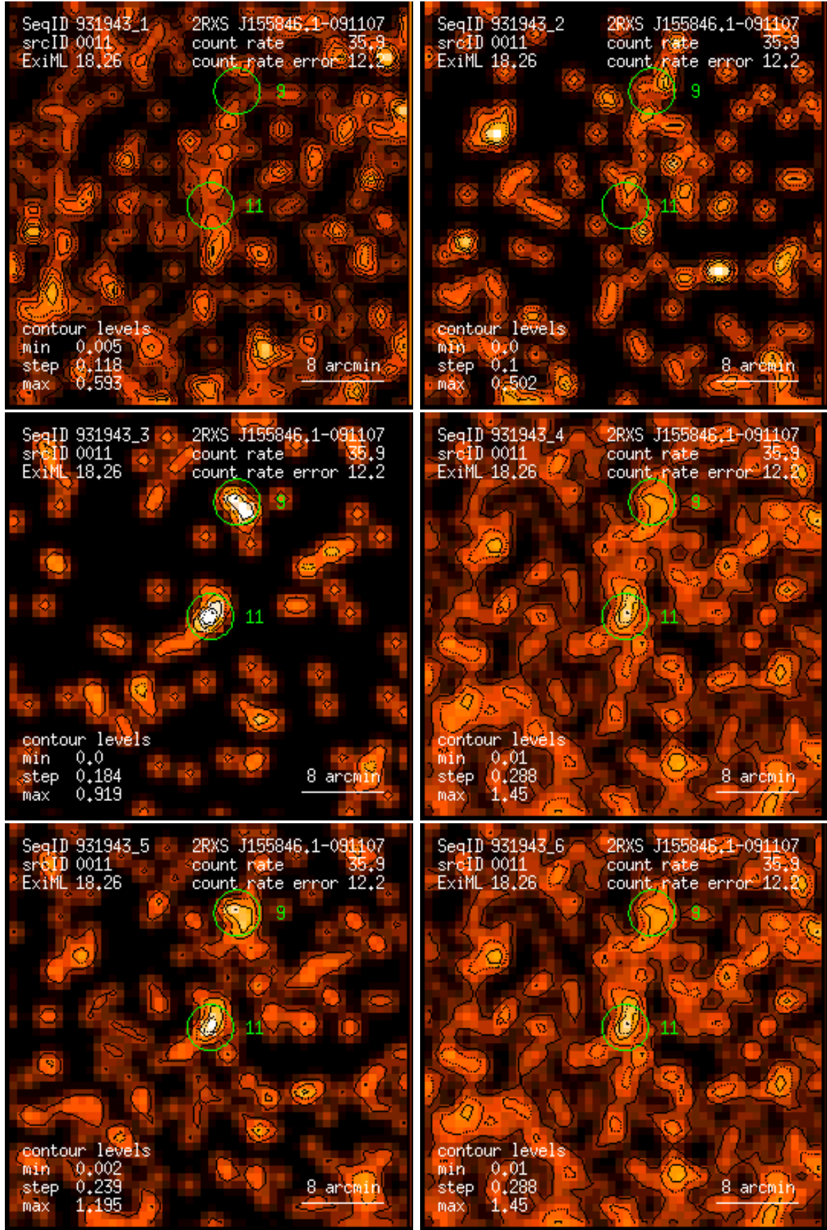
Figure 11: RASS 931943: detection 0011: band rate images, Gaussian filter: (1) PSPC channels 11 – 41, (2) 52 – 90, (3) 91 – 201, (4) 11 – 235, (5) 52 – 201, (6) 11 – 201. Broad band rates in counts/ks. Band rate contour levels in counts/ks/arcmin 2 .
