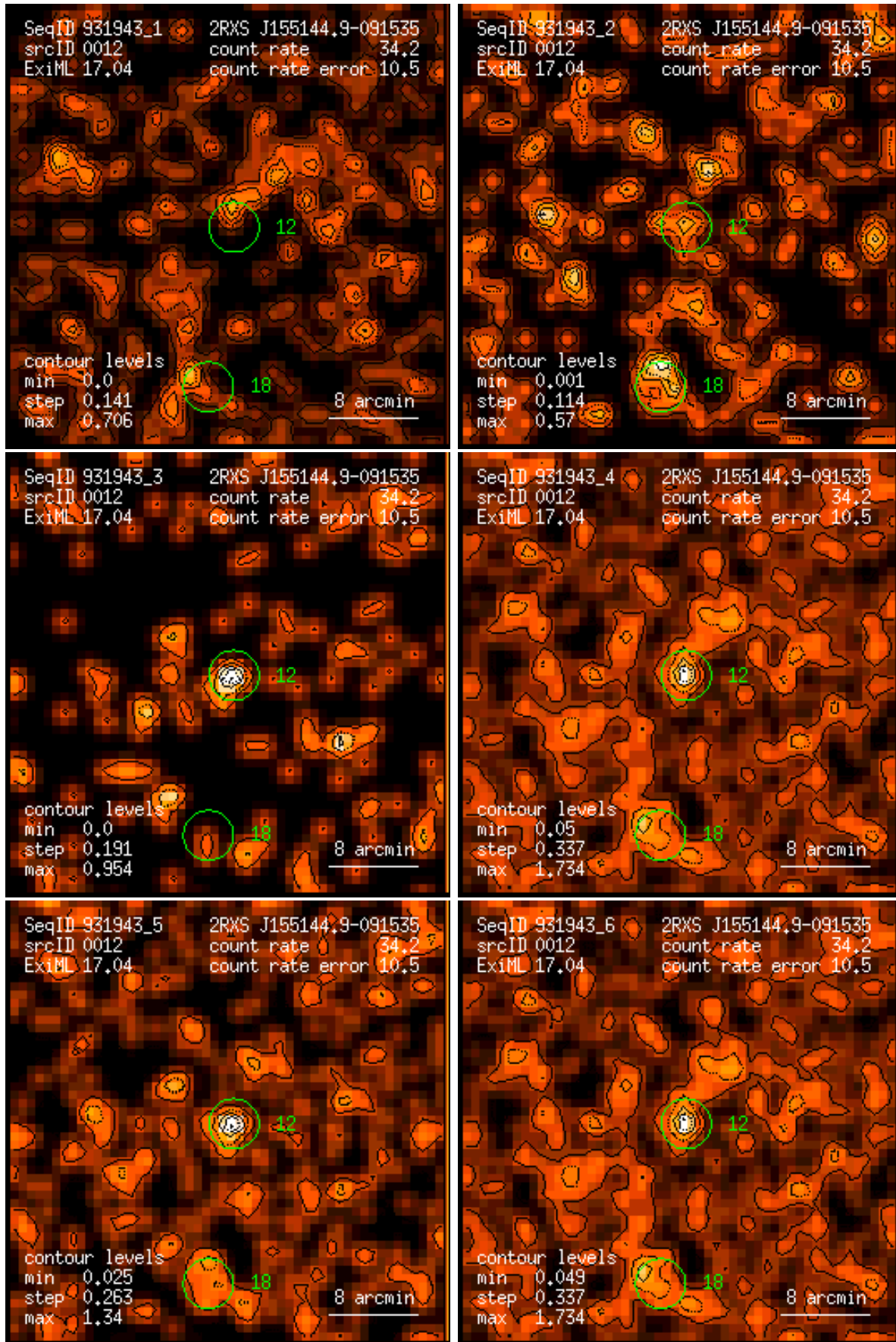
Figure 12: RASS 931943: detection 0012: band rate images, Gaussian filter: (1) PSPC channels 11 – 41, (2) 52 – 90, (3) 91 – 201, (4) 11 – 235, (5) 52 – 201, (6) 11 – 201. Broad band rates in counts/ks. Band rate contour levels in counts/ks/arcmin 2 .
