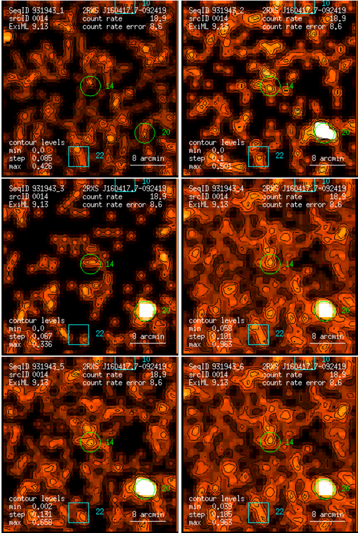
Figure 14: RASS 931943: detection 0014: band rate images, Gaussian filter: (1) PSPC channels 11 – 41, (2) 52 – 90, (3) 91 – 201, (4) 11 – 235, (5) 52 – 201, (6) 11 – 201. Broad band rates in counts/ks. Band rate contour levels in counts/ks/arcmin 2 .
