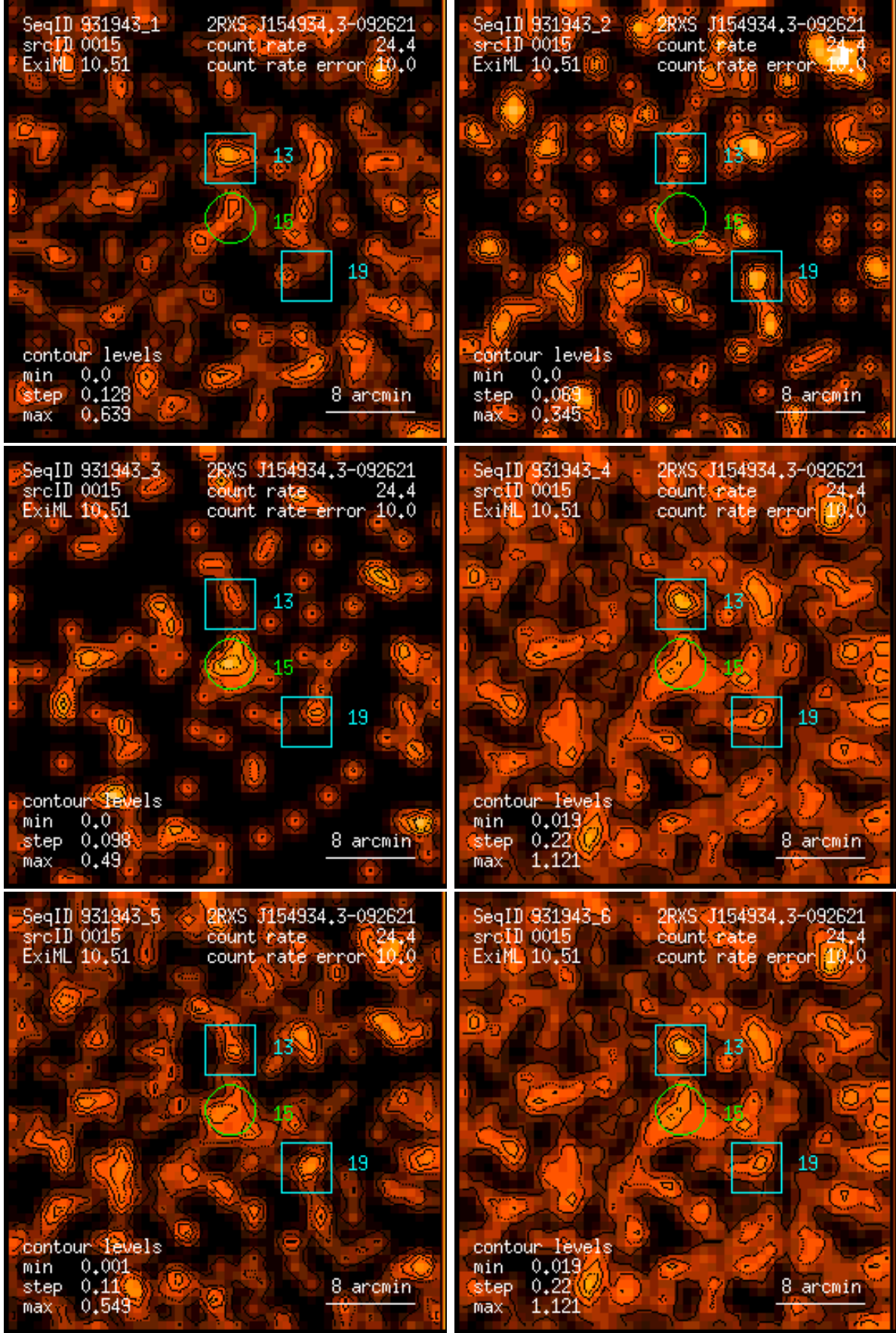
Figure 15: RASS 931943: detection 0015: band rate images, Gaussian filter: (1) PSPC channels 11 – 41, (2) 52 – 90, (3) 91 – 201, (4) 11 – 235, (5) 52 – 201, (6) 11 – 201. Broad band rates in counts/ks. Band rate contour levels in counts/ks/arcmin 2 .
