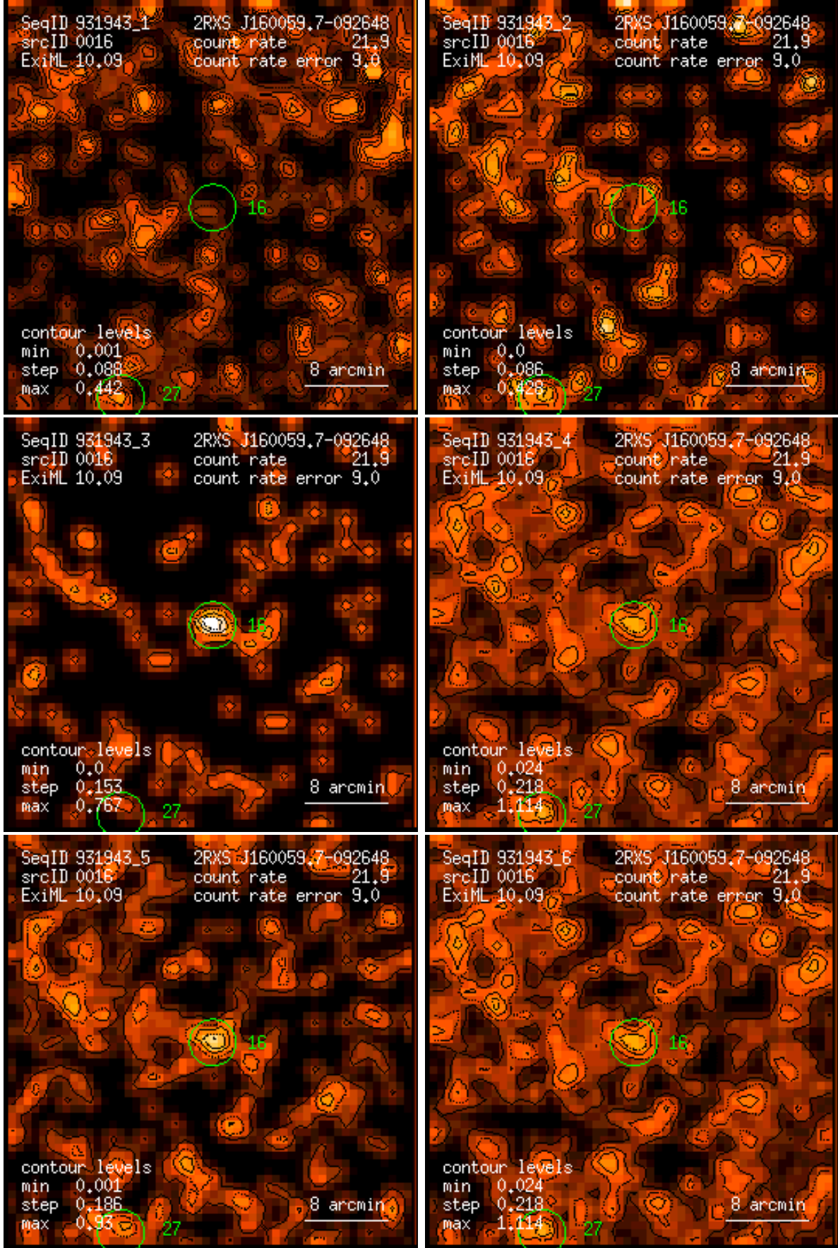
Figure 16: RASS 931943: detection 0016: band rate images, Gaussian filter: (1) PSPC channels 11 – 41, (2) 52 – 90, (3) 91 – 201, (4) 11 – 235, (5) 52 – 201, (6) 11 – 201. Broad band rates in counts/ks. Band rate contour levels in counts/ks/arcmin 2 .
