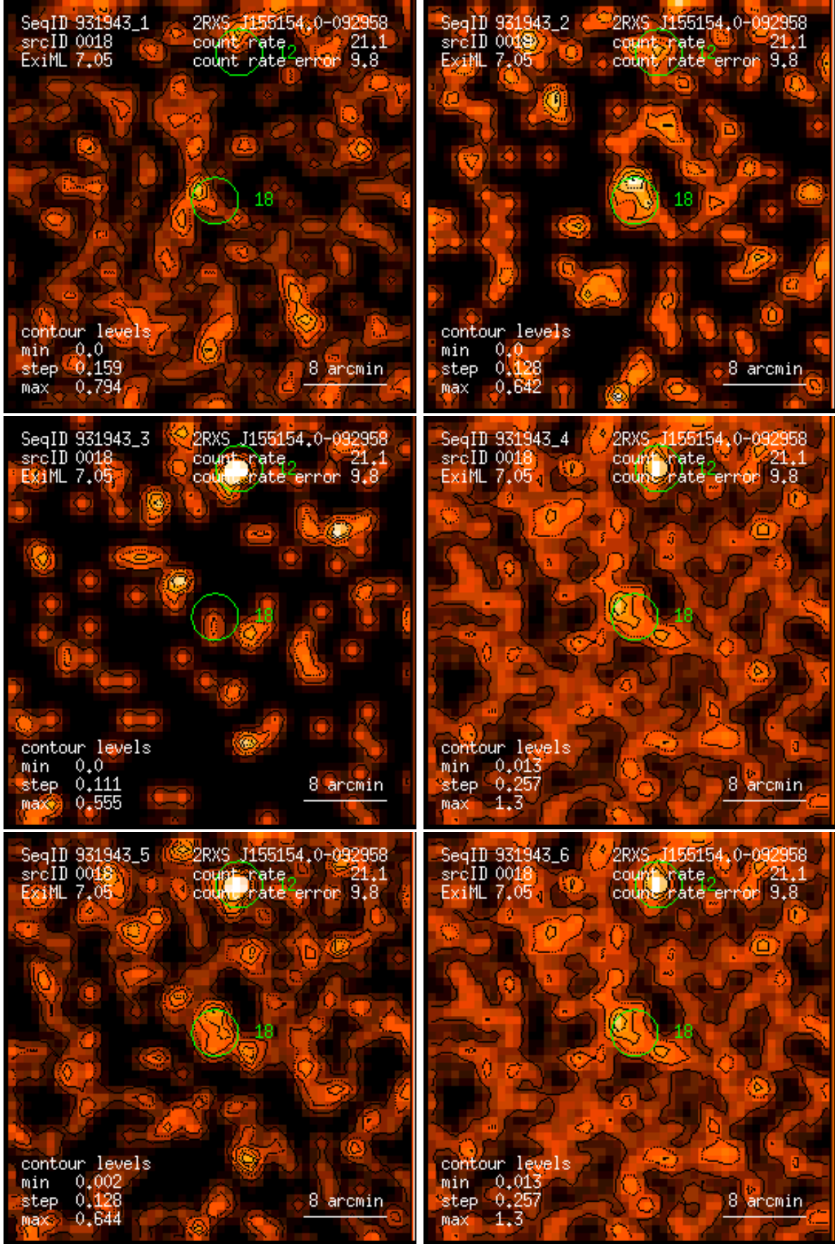
Figure 18: RASS 931943: detection 0018: band rate images, Gaussian filter: (1) PSPC channels 11 – 41, (2) 52 – 90, (3) 91 – 201, (4) 11 – 235, (5) 52 – 201, (6) 11 – 201. Broad band rates in counts/ks. Band rate contour levels in counts/ks/arcmin 2 .
