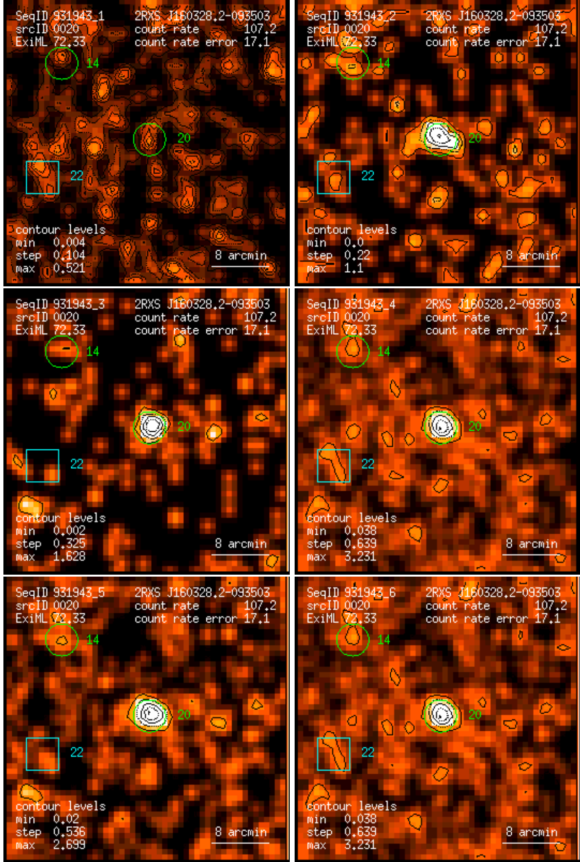
Figure 20: RASS 931943: detection 0020: band rate images, Gaussian filter: (1) PSPC channels 11 – 41, (2) 52 – 90, (3) 91 – 201, (4) 11 – 235, (5) 52 – 201, (6) 11 – 201. Broad band rates in counts/ks. Band rate contour levels in counts/ks/arcmin 2 .
