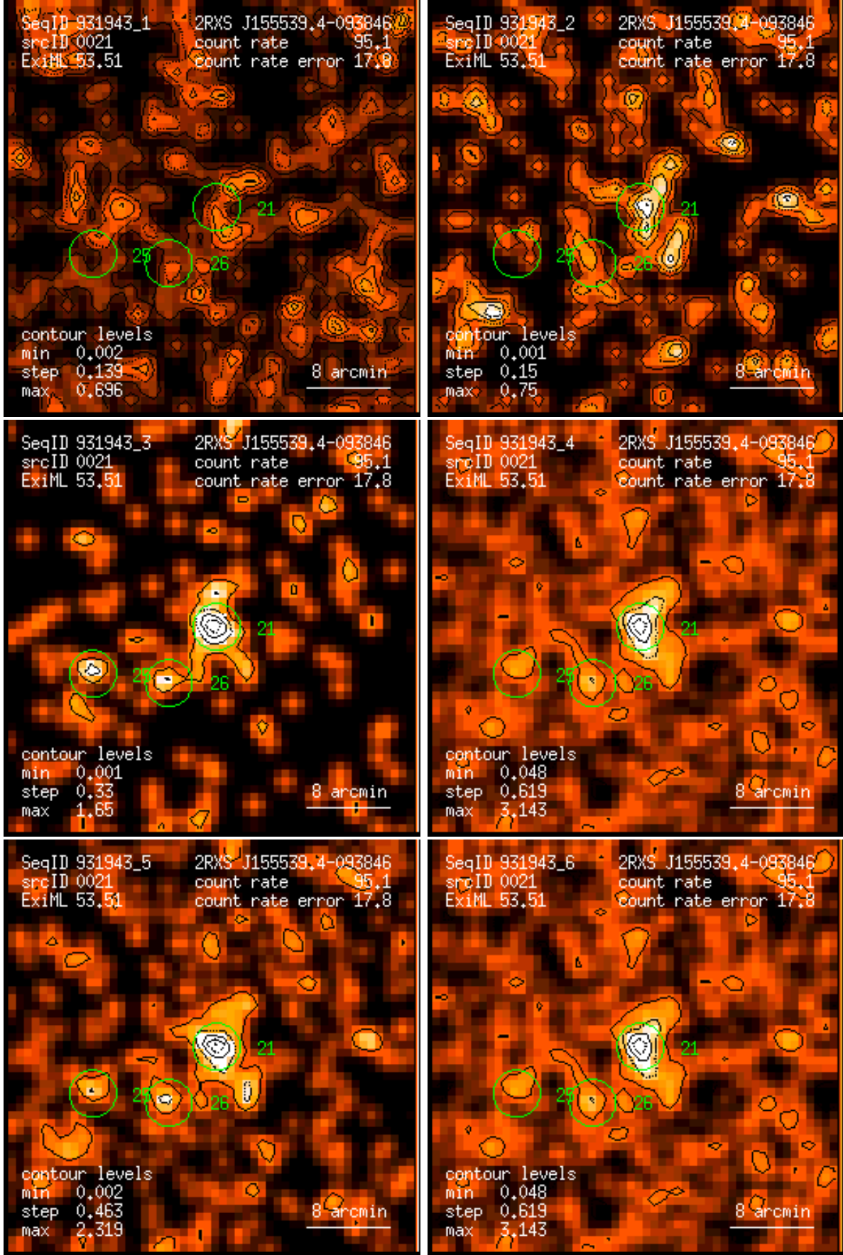
Figure 21: RASS 931943: detection 0021: band rate images, Gaussian filter: (1) PSPC channels 11 – 41, (2) 52 – 90, (3) 91 – 201, (4) 11 – 235, (5) 52 – 201, (6) 11 – 201. Broad band rates in counts/ks. Band rate contour levels in counts/ks/arcmin 2 .
