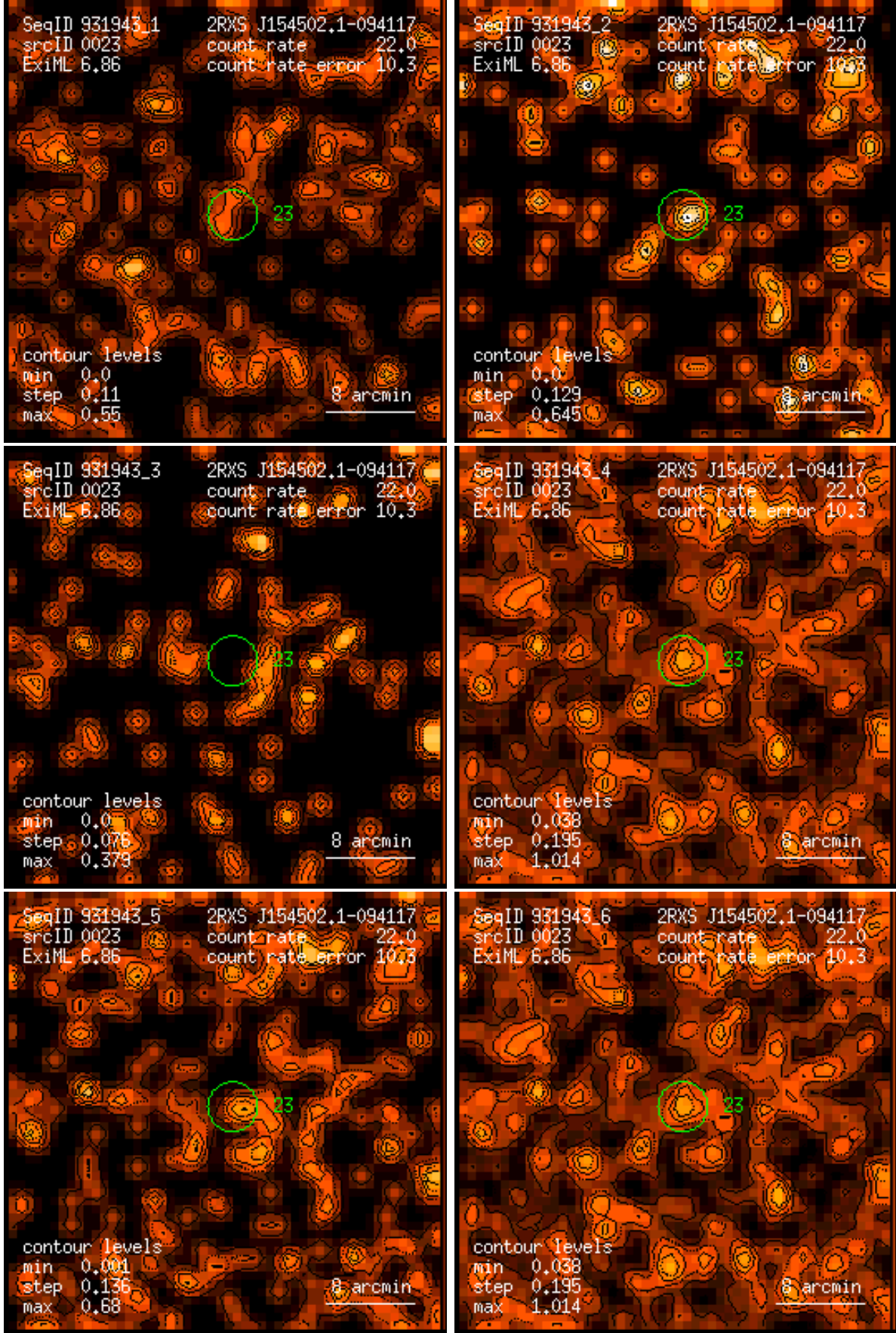
Figure 23: RASS 931943: detection 0023: band rate images, Gaussian filter: (1) PSPC channels 11 – 41, (2) 52 – 90, (3) 91 – 201, (4) 11 – 235, (5) 52 – 201, (6) 11 – 201. Broad band rates in counts/ks. Band rate contour levels in counts/ks/arcmin 2 .
