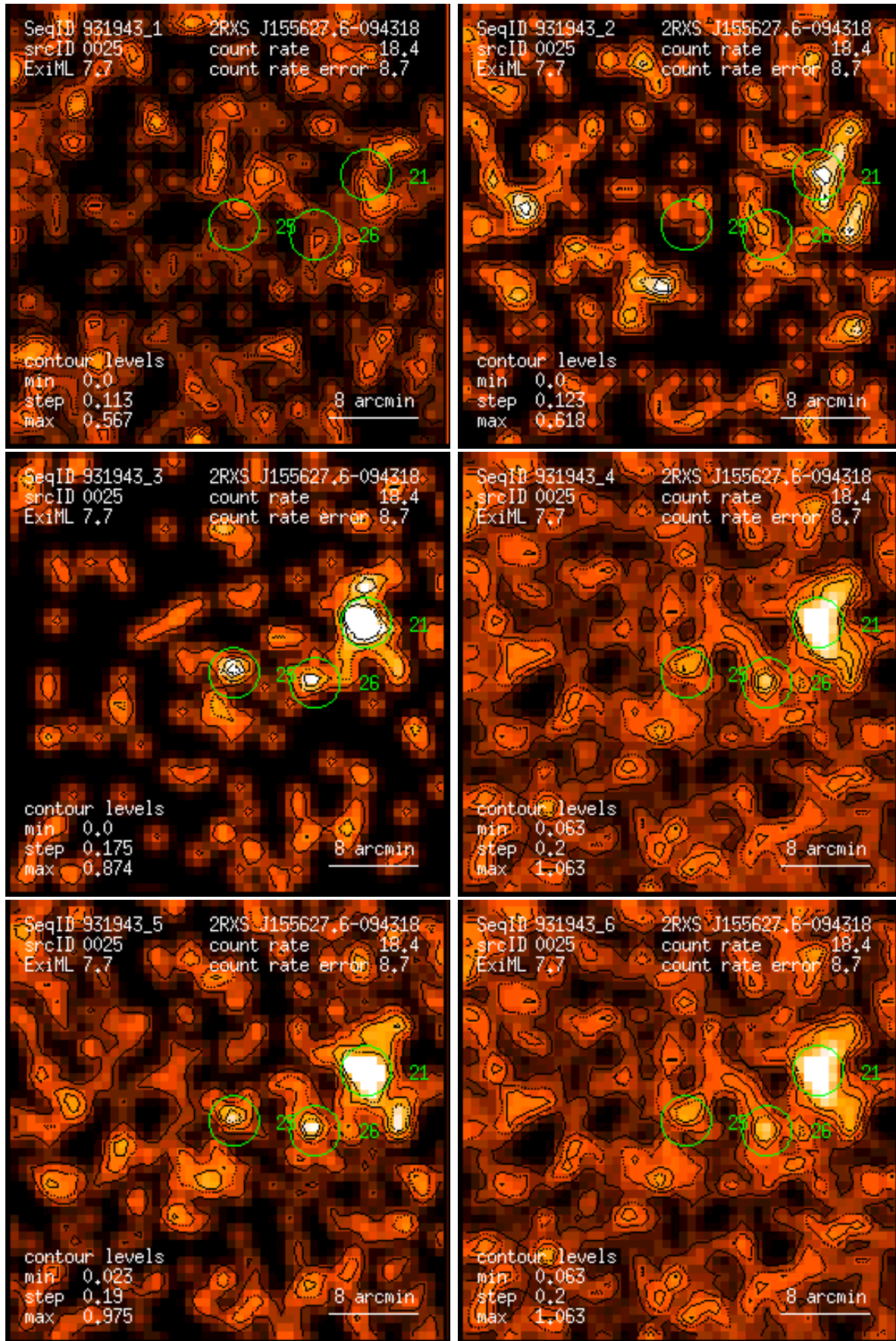
Figure 25: RASS 931943: detection 0025: band rate images, Gaussian filter: (1) PSPC channels 11 – 41, (2) 52 – 90, (3) 91 – 201, (4) 11 – 235, (5) 52 – 201, (6) 11 – 201. Broad band rates in counts/ks. Band rate contour levels in counts/ks/arcmin 2 .
