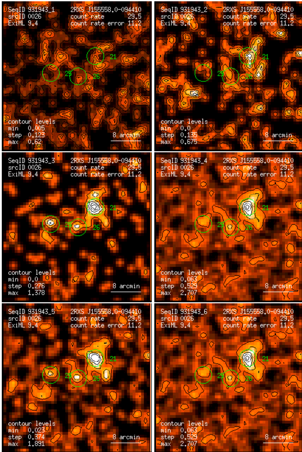
Figure 26: RASS 931943: detection 0026: band rate images, Gaussian filter: (1) PSPC channels 11 – 41, (2) 52 – 90, (3) 91 – 201, (4) 11 – 235, (5) 52 – 201, (6) 11 – 201. Broad band rates in counts/ks. Band rate contour levels in counts/ks/arcmin 2 .
