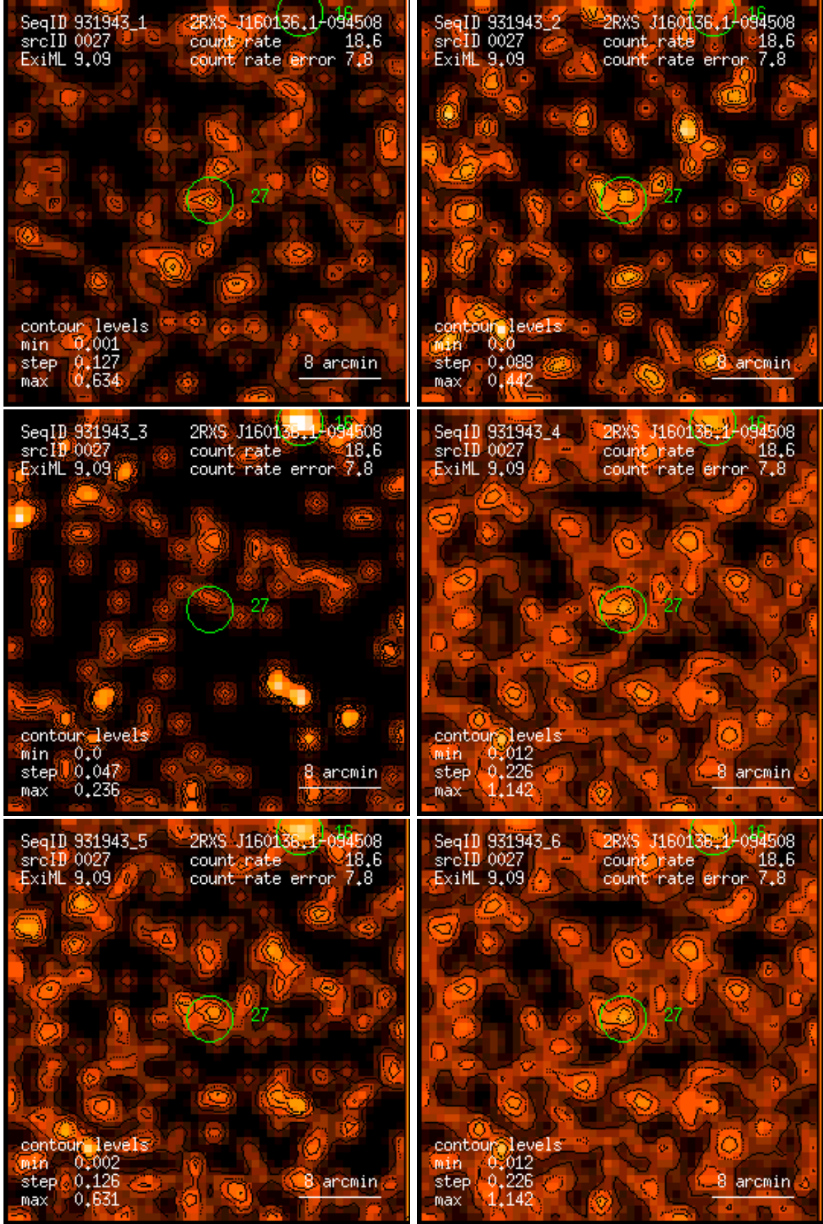
Figure 27: RASS 931943: detection 0027: band rate images, Gaussian filter: (1) PSPC channels 11 – 41, (2) 52 – 90, (3) 91 – 201, (4) 11 – 235, (5) 52 – 201, (6) 11 – 201. Broad band rates in counts/ks. Band rate contour levels in counts/ks/arcmin 2 .
