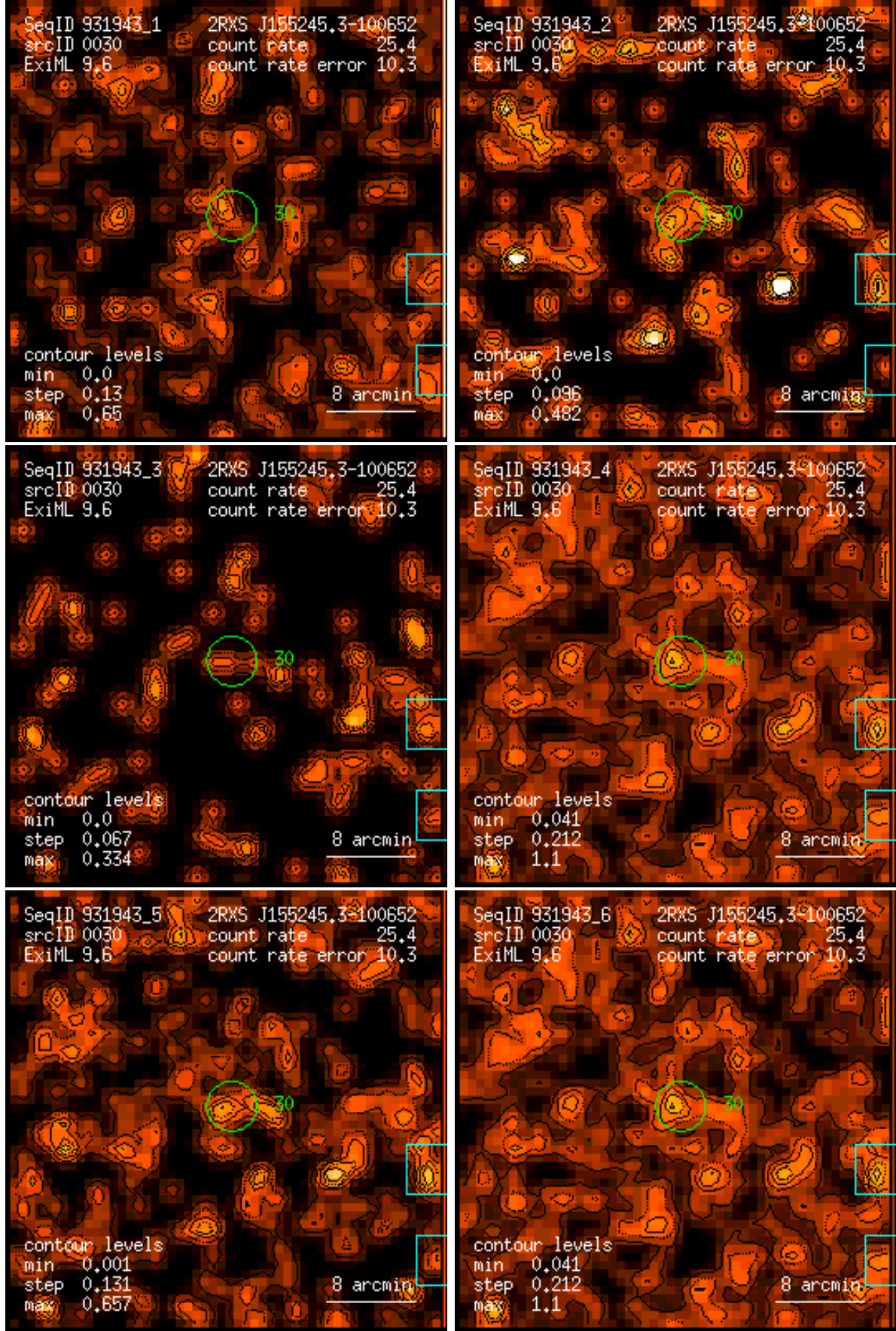
Figure 30: RASS 931943: detection 0030: band rate images, Gaussian filter: (1) PSPC channels 11 – 41, (2) 52 – 90, (3) 91 – 201, (4) 11 – 235, (5) 52 – 201, (6) 11 – 201. Broad band rates in counts/ks. Band rate contour levels in counts/ks/arcmin 2 .
