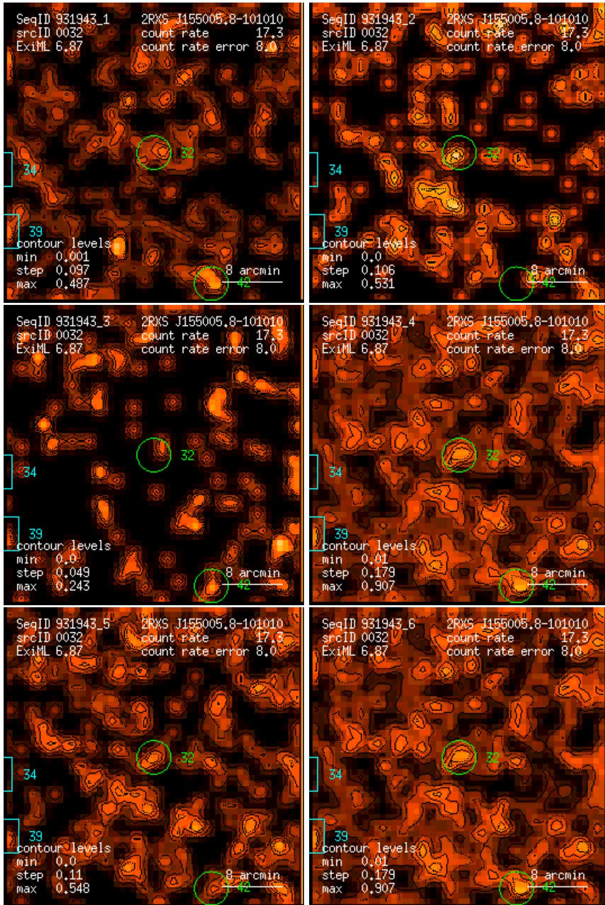
Figure 32: RASS 931943: detection 0032: band rate images, Gaussian filter: (1) PSPC channels 11 – 41, (2) 52 – 90, (3) 91 – 201, (4) 11 – 235, (5) 52 – 201, (6) 11 – 201. Broad band rates in counts/ks. Band rate contour levels in counts/ks/arcmin 2 .
