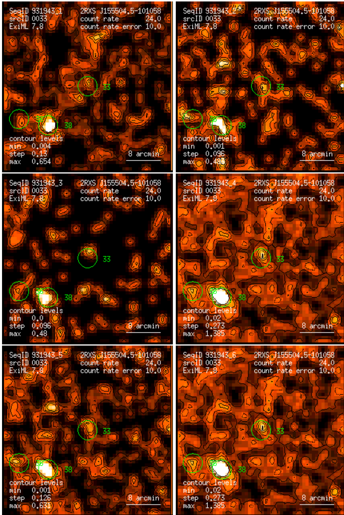
Figure 33: RASS 931943: detection 0033: band rate images, Gaussian filter: (1) PSPC channels 11 – 41, (2) 52 – 90, (3) 91 – 201, (4) 11 – 235, (5) 52 – 201, (6) 11 – 201. Broad band rates in counts/ks. Band rate contour levels in counts/ks/arcmin 2 .
