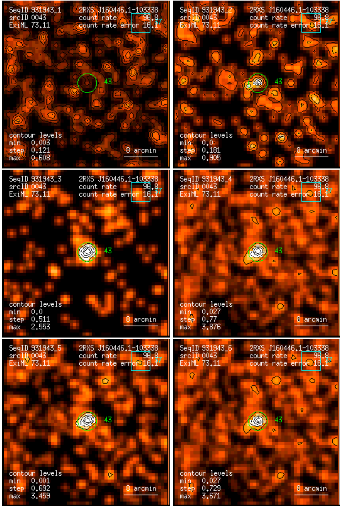
Figure 43: RASS 931943: detection 0043: band rate images, Gaussian filter: (1) PSPC channels 11 – 41, (2) 52 – 90, (3) 91 – 201, (4) 11 – 235, (5) 52 – 201, (6) 11 – 201. Broad band rates in counts/ks. Band rate contour levels in counts/ks/arcmin 2 .
