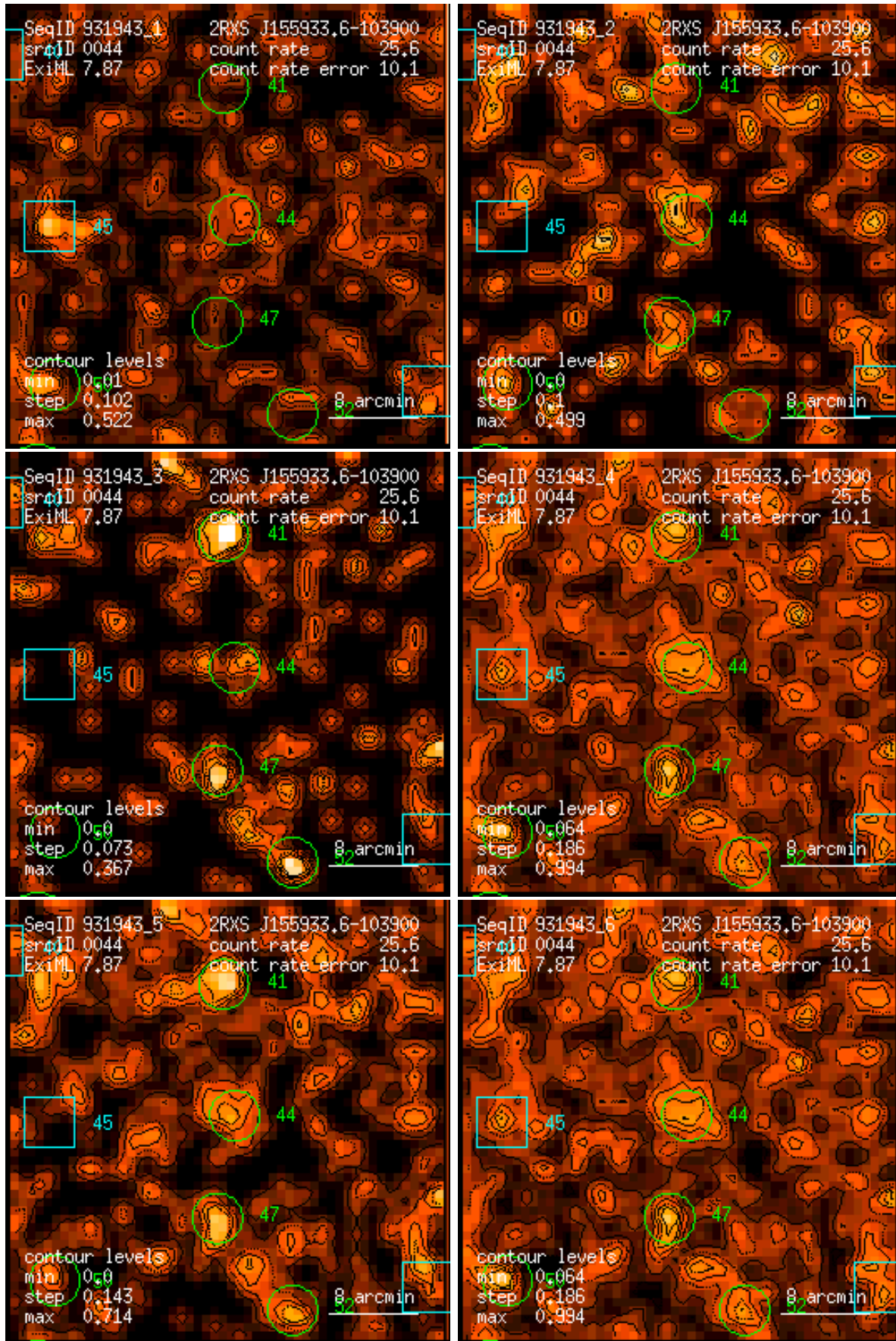
Figure 44: RASS 931943: detection 0044: band rate images, Gaussian filter: (1) PSPC channels 11 – 41, (2) 52 – 90, (3) 91 – 201, (4) 11 – 235, (5) 52 – 201, (6) 11 – 201. Broad band rates in counts/ks. Band rate contour levels in counts/ks/arcmin 2 .
