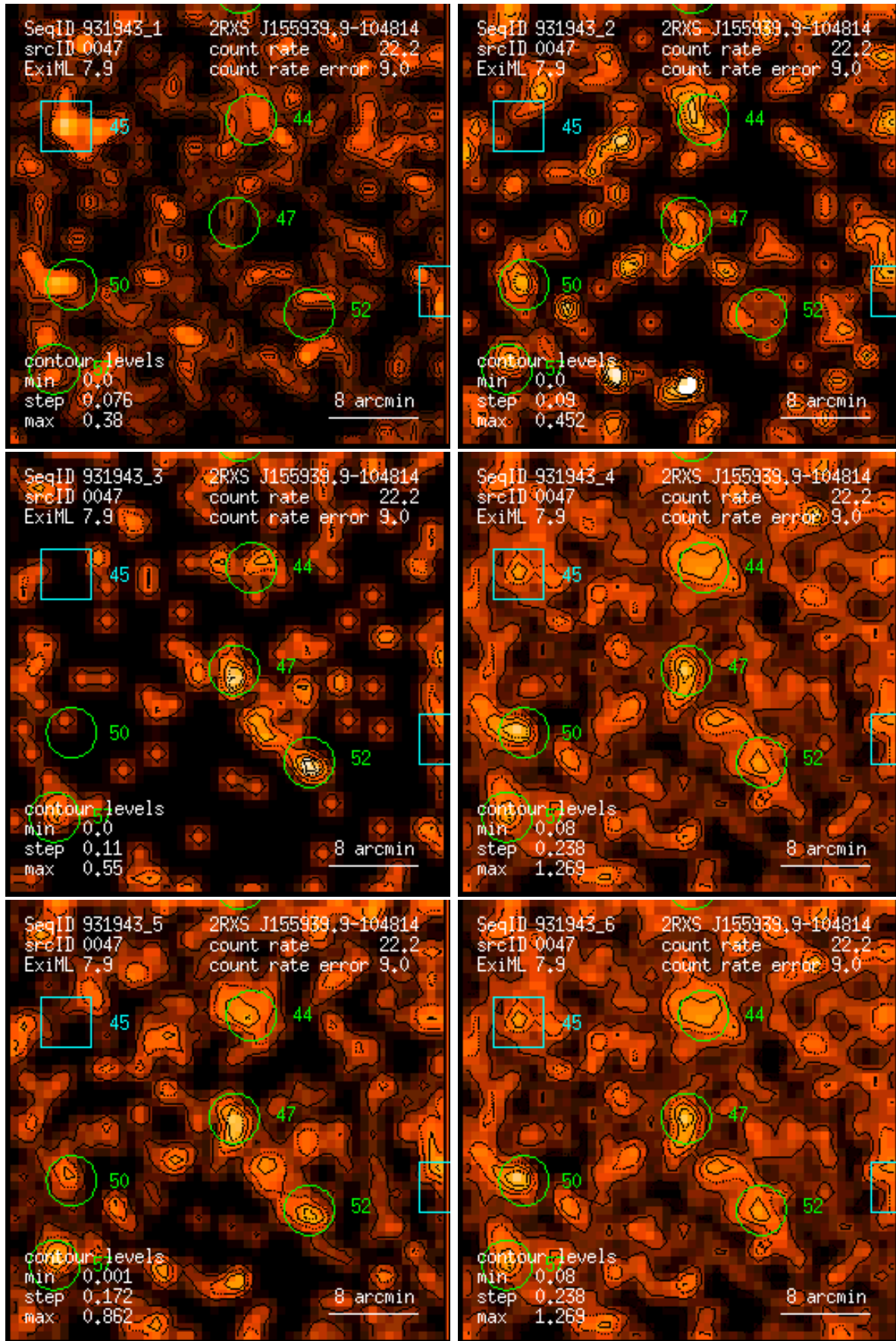
Figure 47: RASS 931943: detection 0047: band rate images, Gaussian filter: (1) PSPC channels 11 – 41, (2) 52 – 90, (3) 91 – 201, (4) 11 – 235, (5) 52 – 201, (6) 11 – 201. Broad band rates in counts/ks. Band rate contour levels in counts/ks/arcmin 2 .
