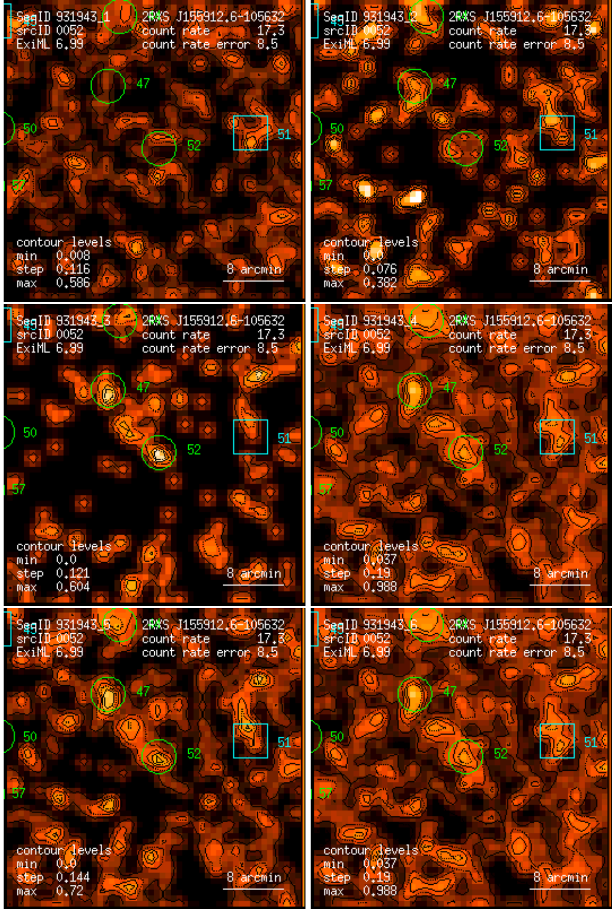
Figure 52: RASS 931943: detection 0052: band rate images, Gaussian filter: (1) PSPC channels 11 – 41, (2) 52 – 90, (3) 91 – 201, (4) 11 – 235, (5) 52 – 201, (6) 11 – 201. Broad band rates in counts/ks. Band rate contour levels in counts/ks/arcmin 2 .
