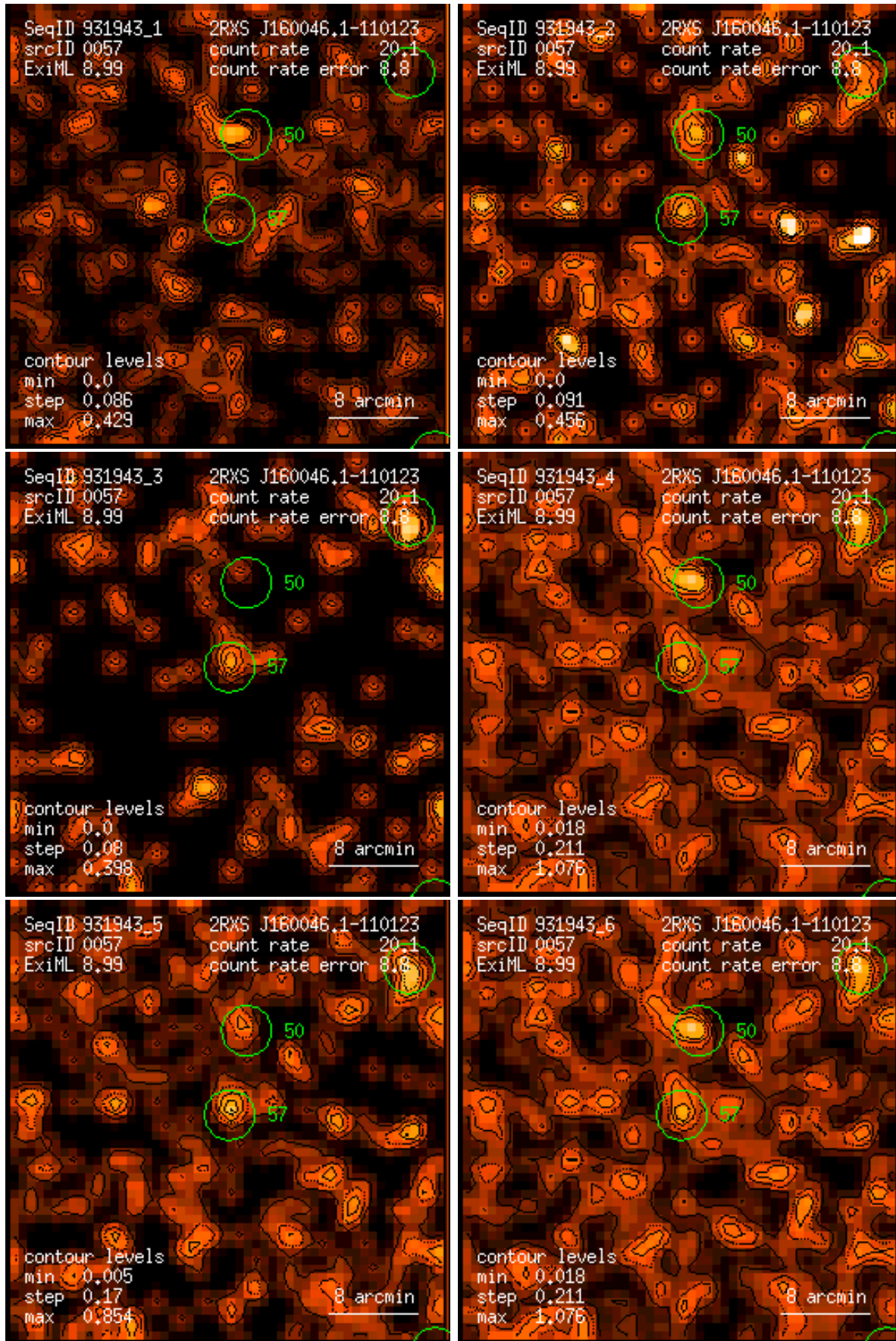
Figure 57: RASS 931943: detection 0057: band rate images, Gaussian filter: (1) PSPC channels 11 – 41, (2) 52 – 90, (3) 91 – 201, (4) 11 – 235, (5) 52 – 201, (6) 11 – 201. Broad band rates in counts/ks. Band rate contour levels in counts/ks/arcmin 2 .
