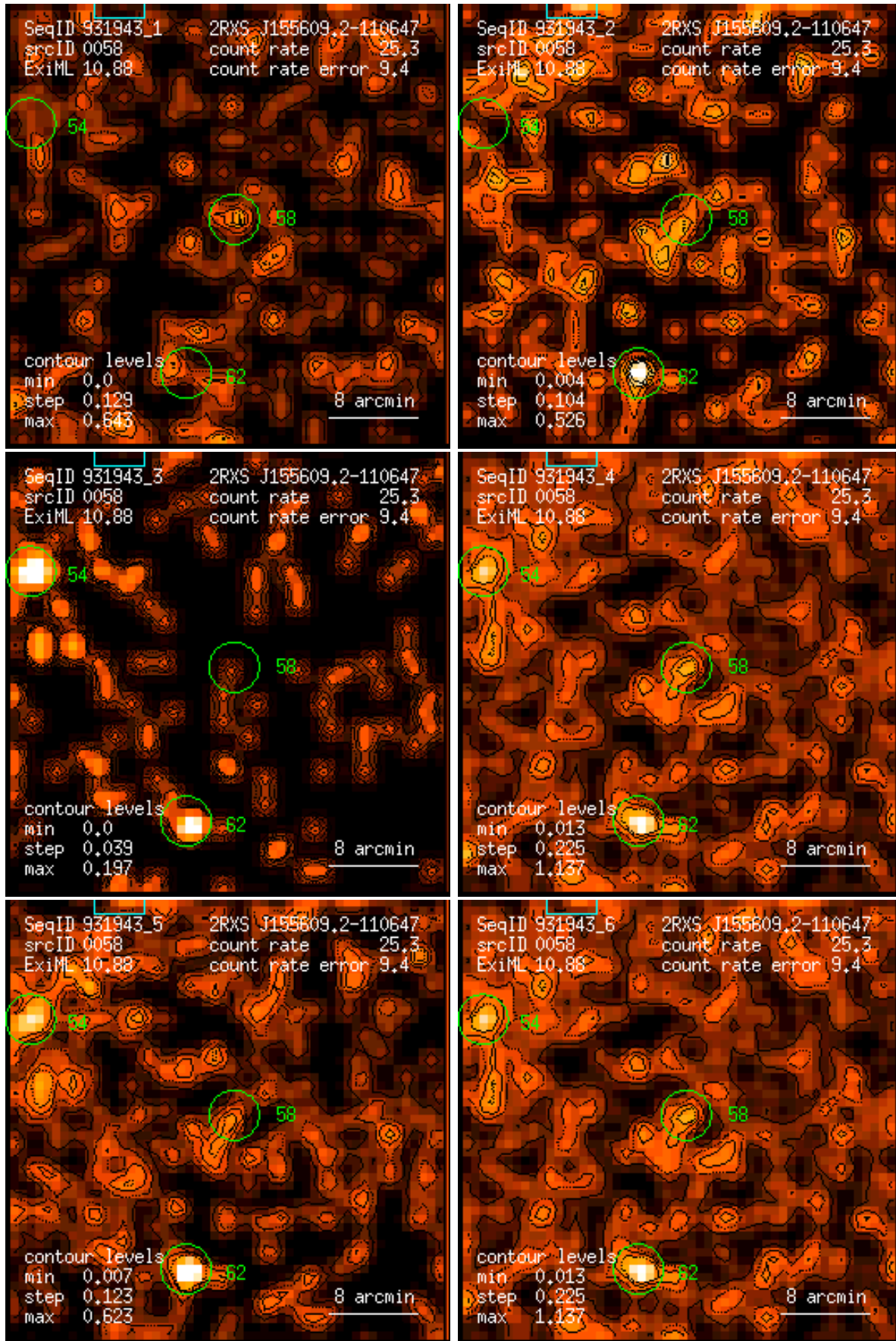
Figure 58: RASS 931943: detection 0058: band rate images, Gaussian filter: (1) PSPC channels 11 – 41, (2) 52 – 90, (3) 91 – 201, (4) 11 – 235, (5) 52 – 201, (6) 11 – 201. Broad band rates in counts/ks. Band rate contour levels in counts/ks/arcmin 2 .
