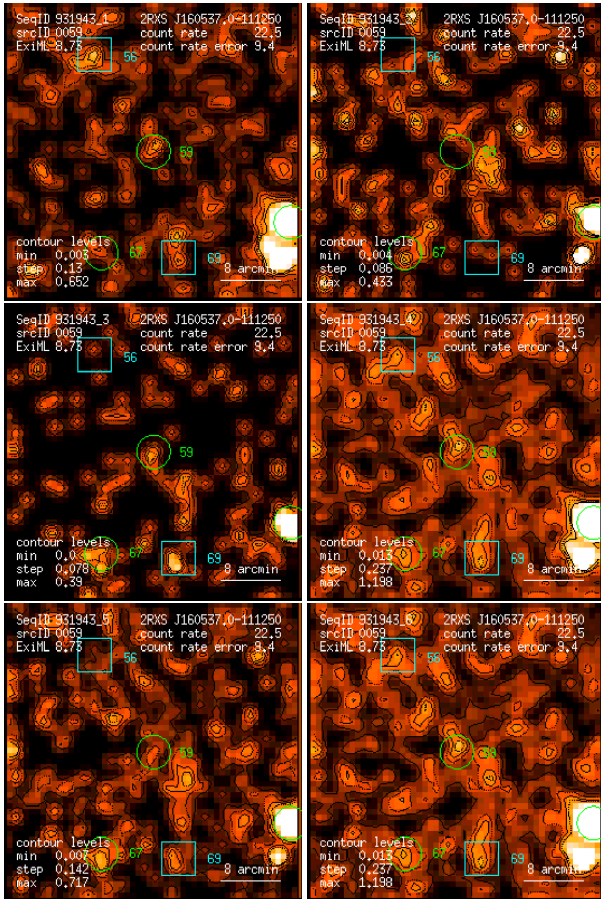
Figure 59: RASS 931943: detection 0059: band rate images, Gaussian filter: (1) PSPC channels 11 – 41, (2) 52 – 90, (3) 91 – 201, (4) 11 – 235, (5) 52 – 201, (6) 11 – 201. Broad band rates in counts/ks. Band rate contour levels in counts/ks/arcmin 2 .
