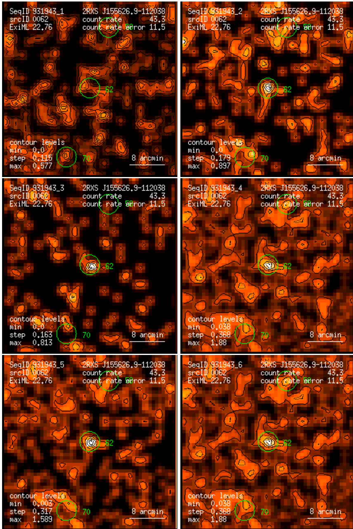
Figure 62: RASS 931943: detection 0062: band rate images, Gaussian filter: (1) PSPC channels 11 – 41, (2) 52 – 90, (3) 91 – 201, (4) 11 – 235, (5) 52 – 201, (6) 11 – 201. Broad band rates in counts/ks. Band rate contour levels in counts/ks/arcmin 2 .
