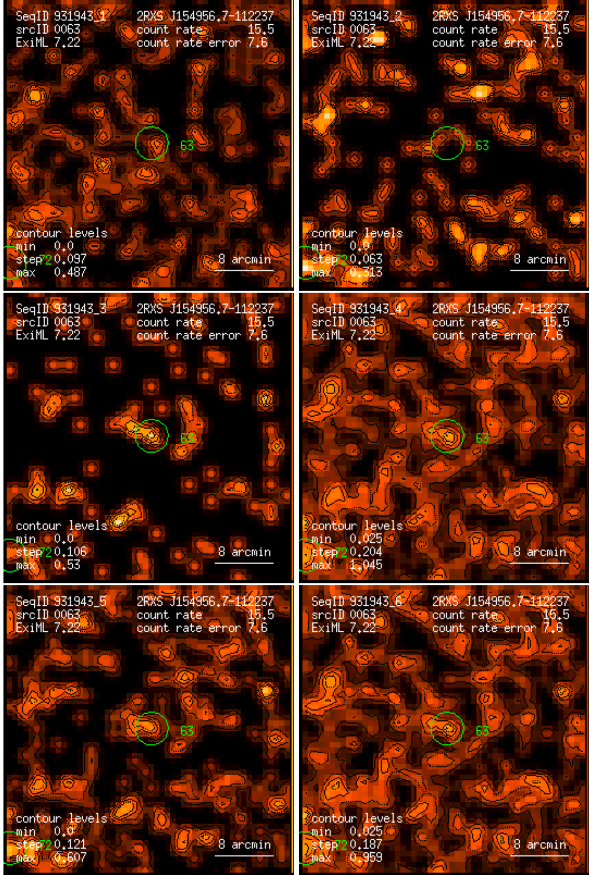
Figure 63: RASS 931943: detection 0063: band rate images, Gaussian filter: (1) PSPC channels 11 – 41, (2) 52 – 90, (3) 91 – 201, (4) 11 – 235, (5) 52 – 201, (6) 11 – 201. Broad band rates in counts/ks. Band rate contour levels in counts/ks/arcmin 2 .
