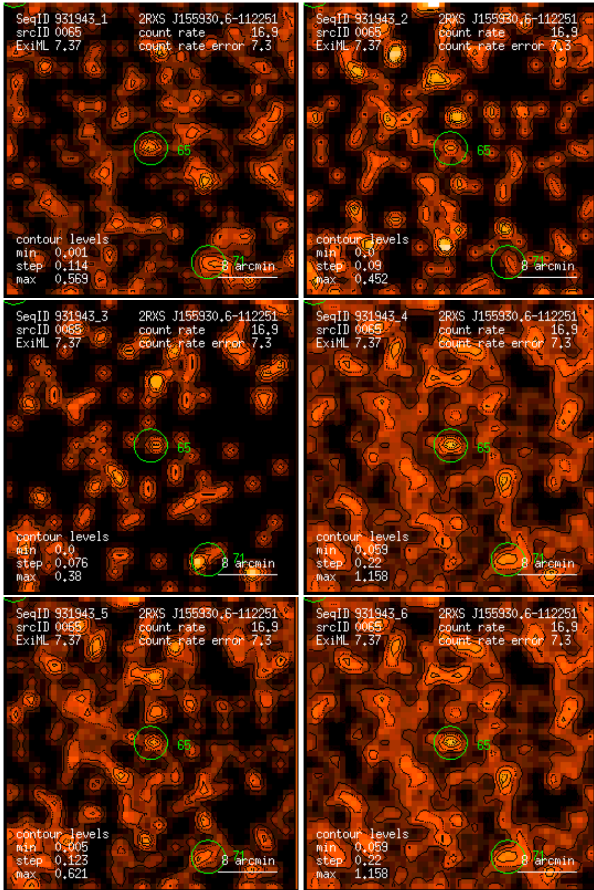
Figure 65: RASS 931943: detection 0065: band rate images, Gaussian filter: (1) PSPC channels 11 – 41, (2) 52 – 90, (3) 91 – 201, (4) 11 – 235, (5) 52 – 201, (6) 11 – 201. Broad band rates in counts/ks. Band rate contour levels in counts/ks/arcmin 2 .
