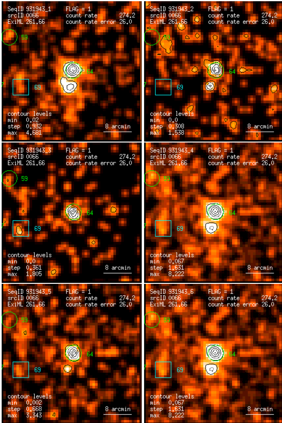
Figure 66: RASS 931943: detection 0066: band rate images, Gaussian filter: (1) PSPC channels 11 – 41, (2) 52 – 90, (3) 91 – 201, (4) 11 – 235, (5) 52 – 201, (6) 11 – 201. Broad band rates in counts/ks. Band rate contour levels in counts/ks/arcmin 2 .
