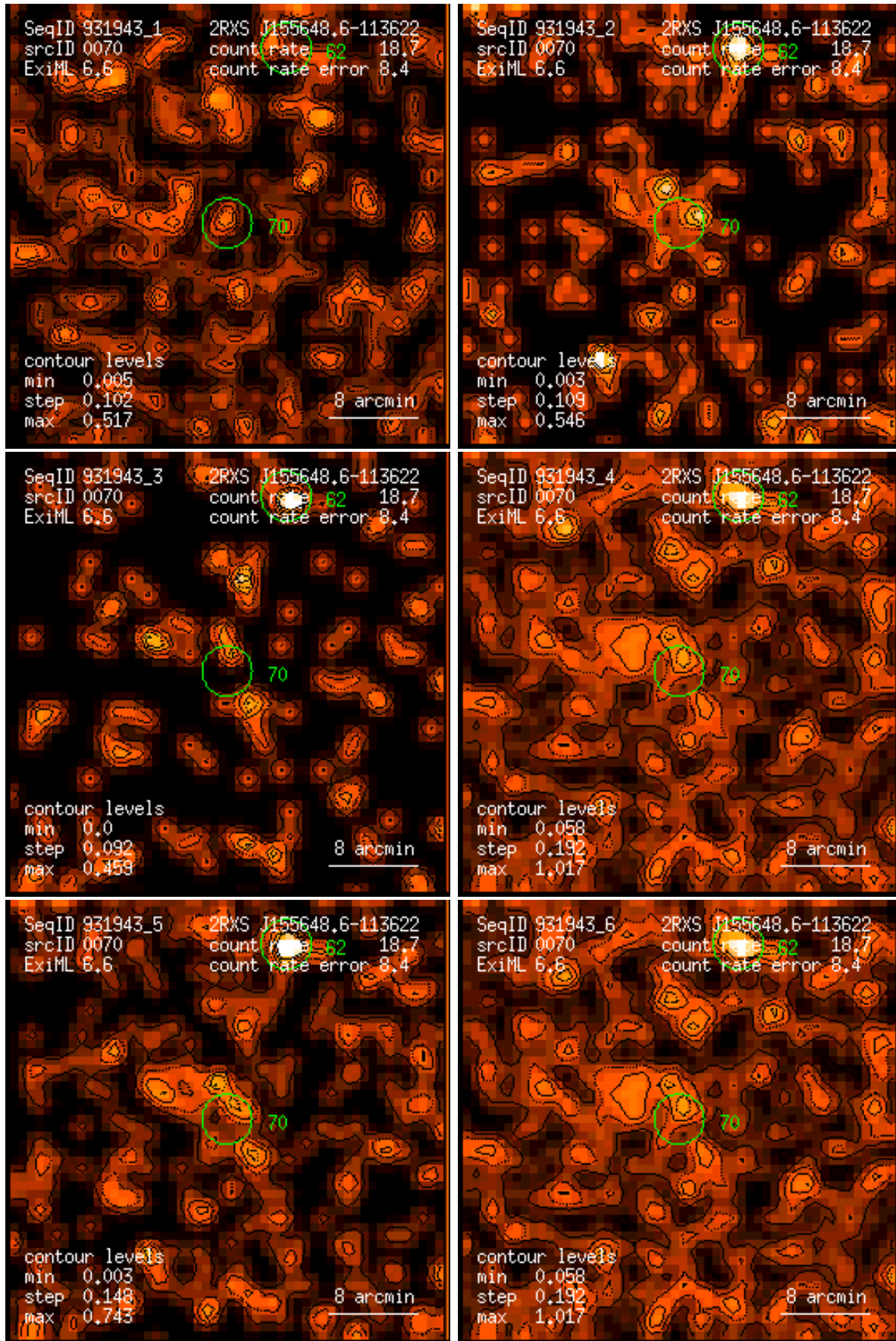
Figure 70: RASS 931943: detection 0070: band rate images, Gaussian filter: (1) PSPC channels 11 – 41, (2) 52 – 90, (3) 91 – 201, (4) 11 – 235, (5) 52 – 201, (6) 11 – 201. Broad band rates in counts/ks. Band rate contour levels in counts/ks/arcmin 2 .
