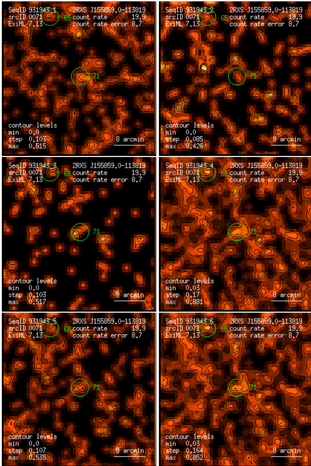
Figure 71: RASS 931943: detection 0071: band rate images, Gaussian filter: (1) PSPC channels 11 – 41, (2) 52 – 90, (3) 91 – 201, (4) 11 – 235, (5) 52 – 201, (6) 11 – 201. Broad band rates in counts/ks. Band rate contour levels in counts/ks/arcmin 2 .
