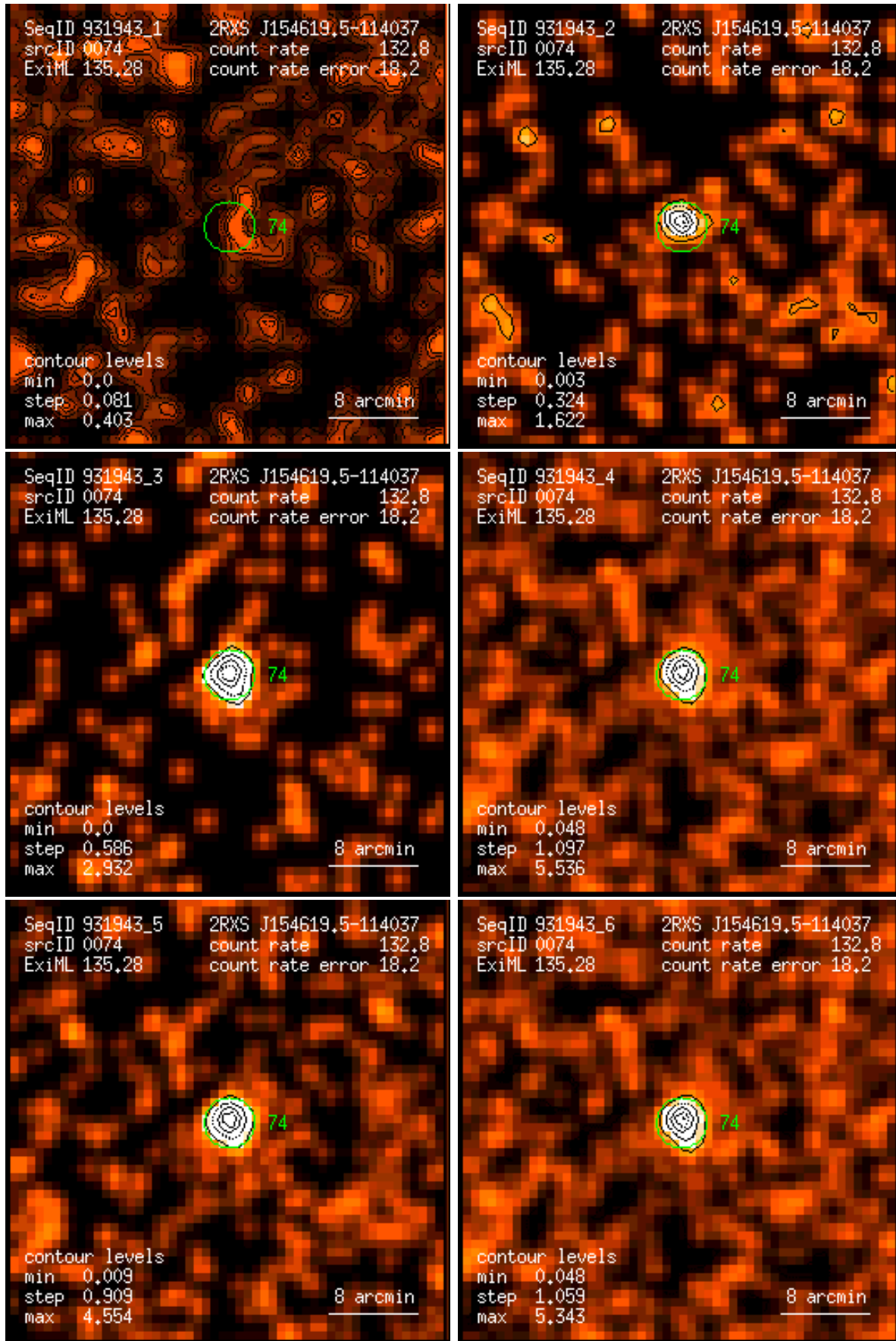
Figure 74: RASS 931943: detection 0074: band rate images, Gaussian filter: (1) PSPC channels 11 – 41, (2) 52 – 90, (3) 91 – 201, (4) 11 – 235, (5) 52 – 201, (6) 11 – 201. Broad band rates in counts/ks. Band rate contour levels in counts/ks/arcmin 2 .
