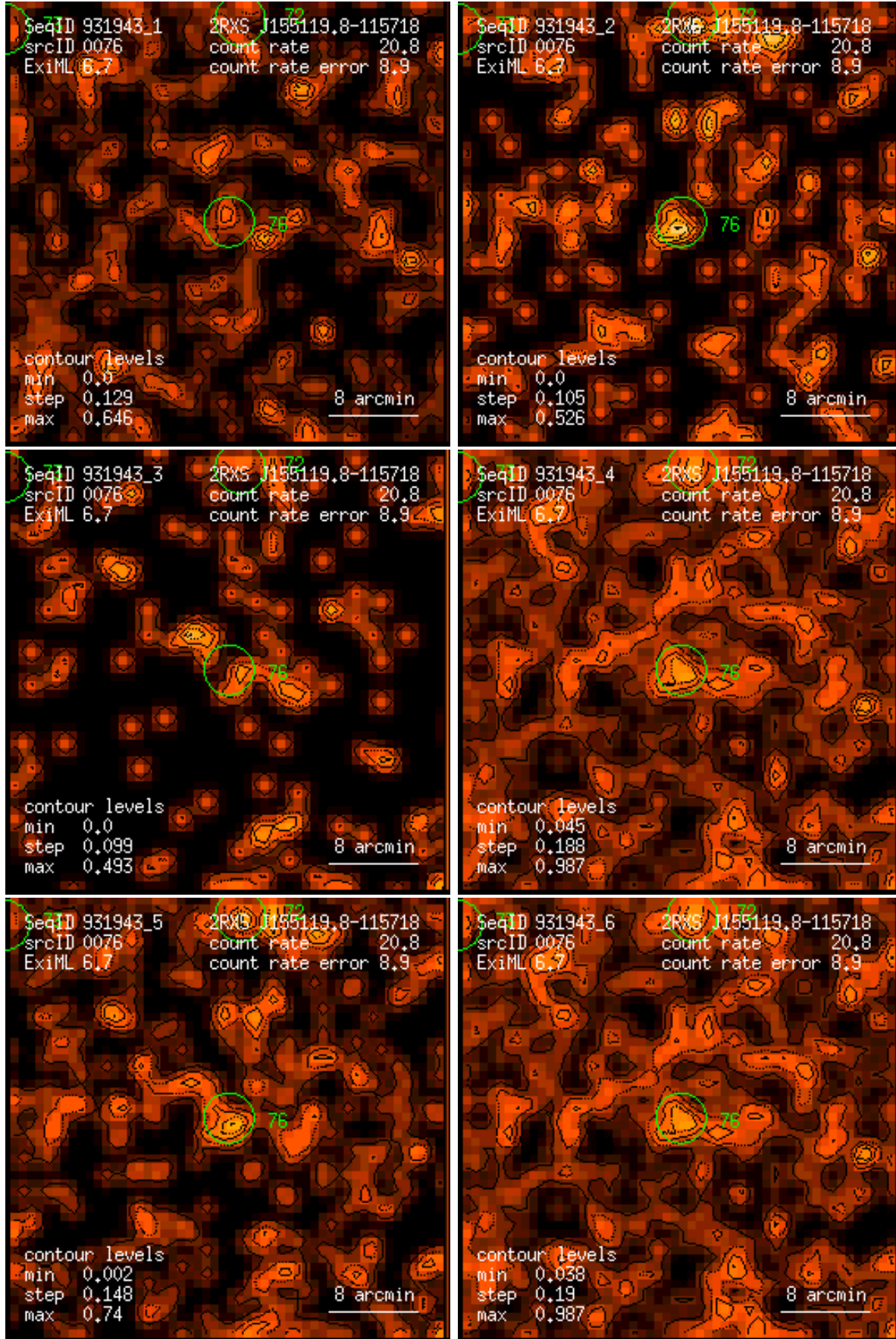
Figure 76: RASS 931943: detection 0076: band rate images, Gaussian filter: (1) PSPC channels 11 – 41, (2) 52 – 90, (3) 91 – 201, (4) 11 – 235, (5) 52 – 201, (6) 11 – 201. Broad band rates in counts/ks. Band rate contour levels in counts/ks/arcmin 2 .
