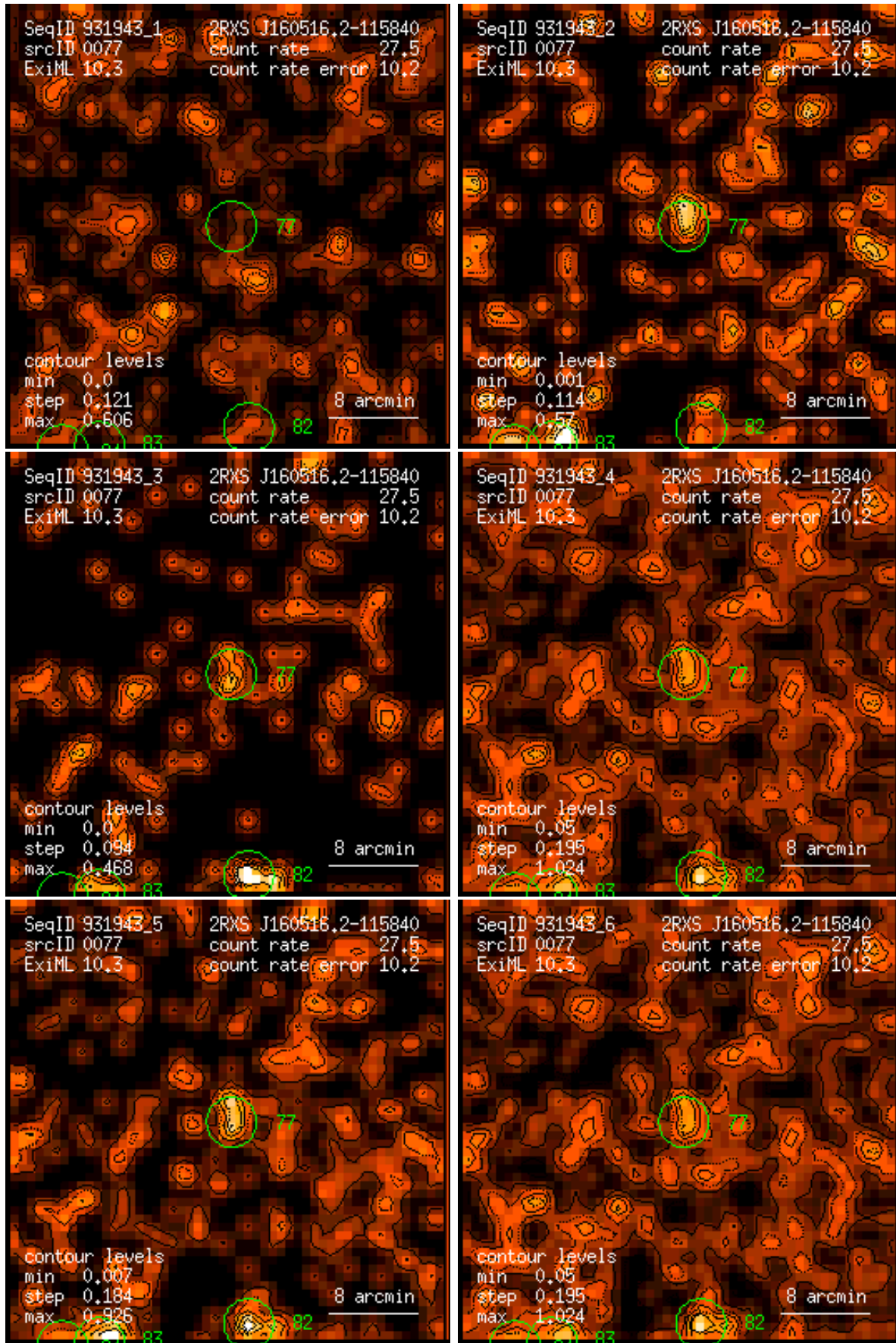
Figure 77: RASS 931943: detection 0077: band rate images, Gaussian filter: (1) PSPC channels 11 – 41, (2) 52 – 90, (3) 91 – 201, (4) 11 – 235, (5) 52 – 201, (6) 11 – 201. Broad band rates in counts/ks. Band rate contour levels in counts/ks/arcmin 2 .
