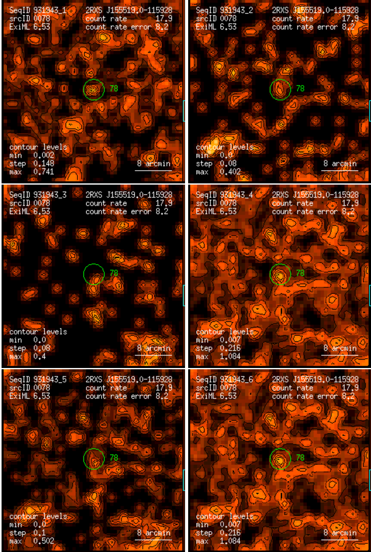
Figure 78: RASS 931943: detection 0078: band rate images, Gaussian filter: (1) PSPC channels 11 – 41, (2) 52 – 90, (3) 91 – 201, (4) 11 – 235, (5) 52 – 201, (6) 11 – 201. Broad band rates in counts/ks. Band rate contour levels in counts/ks/arcmin 2 .
