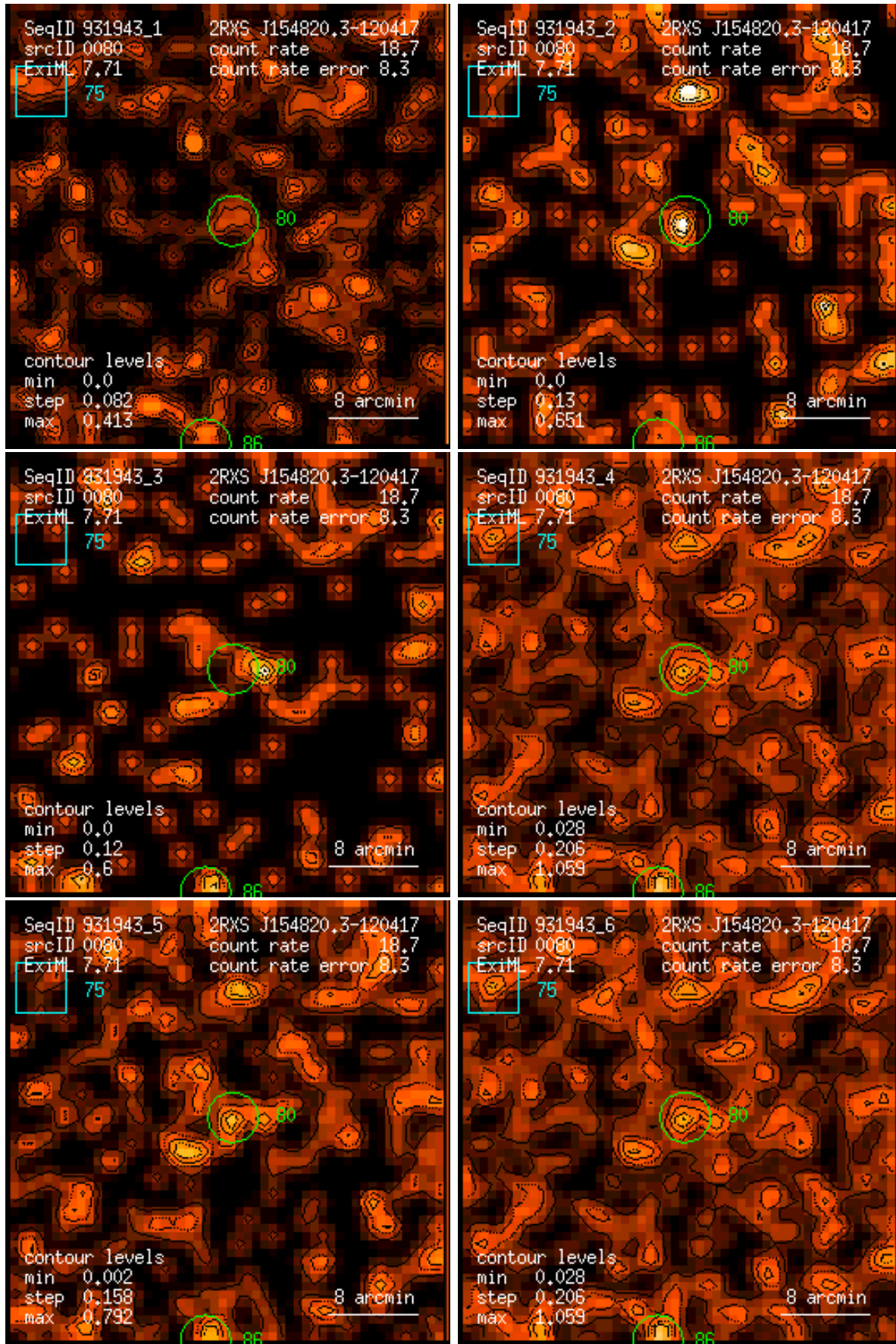
Figure 80: RASS 931943: detection 0080: band rate images, Gaussian filter: (1) PSPC channels 11 – 41, (2) 52 – 90, (3) 91 – 201, (4) 11 – 235, (5) 52 – 201, (6) 11 – 201. Broad band rates in counts/ks. Band rate contour levels in counts/ks/arcmin 2 .
