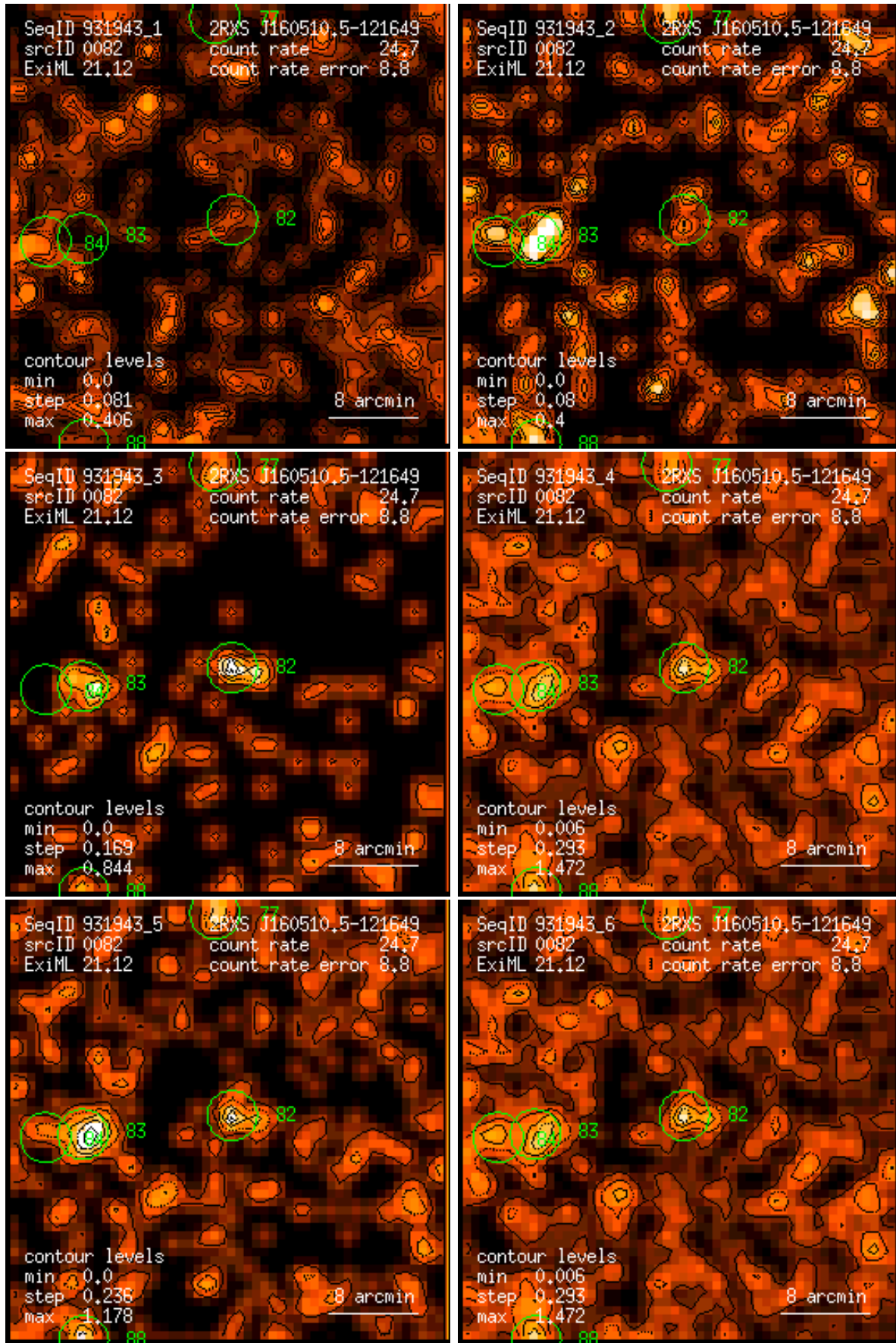
Figure 82: RASS 931943: detection 0082: band rate images, Gaussian filter: (1) PSPC channels 11 – 41, (2) 52 – 90, (3) 91 – 201, (4) 11 – 235, (5) 52 – 201, (6) 11 – 201. Broad band rates in counts/ks. Band rate contour levels in counts/ks/arcmin 2 .
